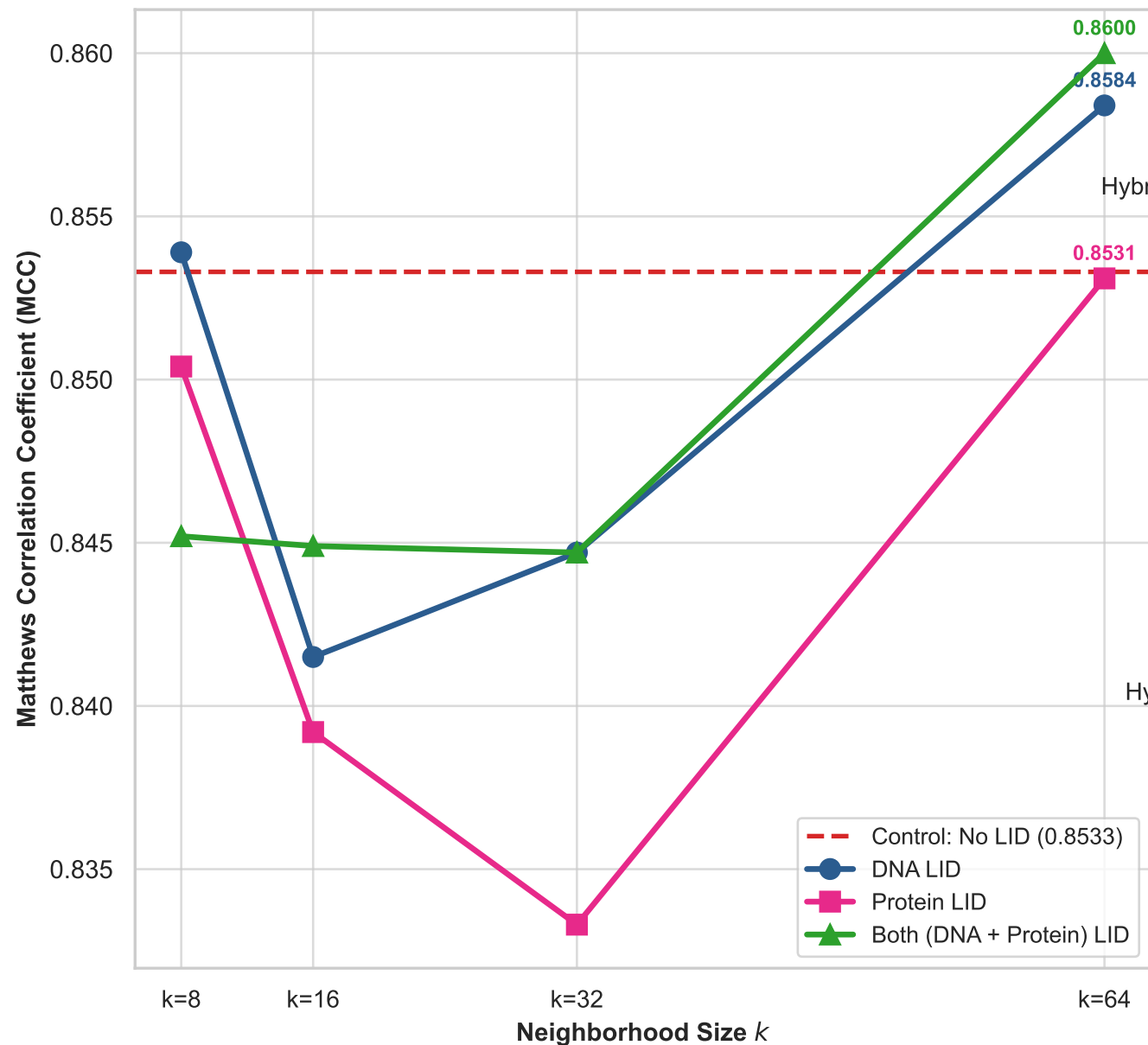
(A) LID Neighborhood Size k Ablation (ClinVarHQ)
