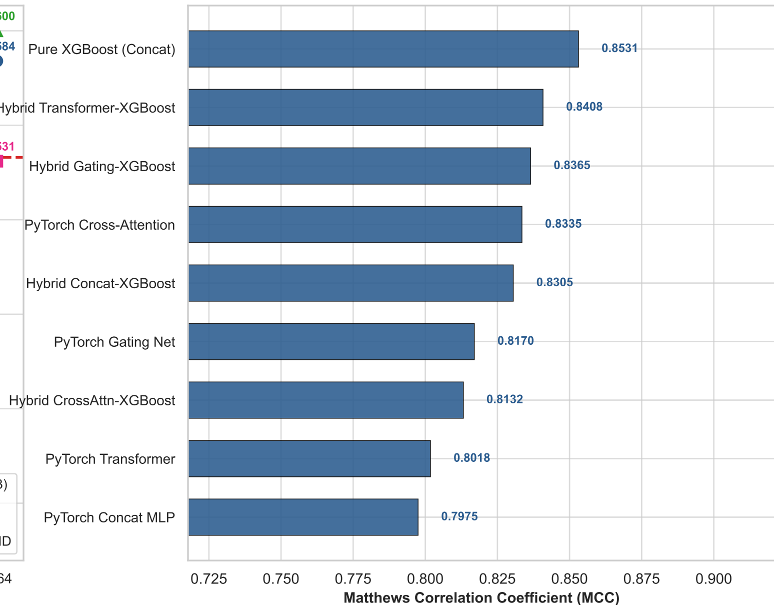
(B) Neural vs Hybrid vs Pure Architectures (ClinVarHQ - DNA k=32)
