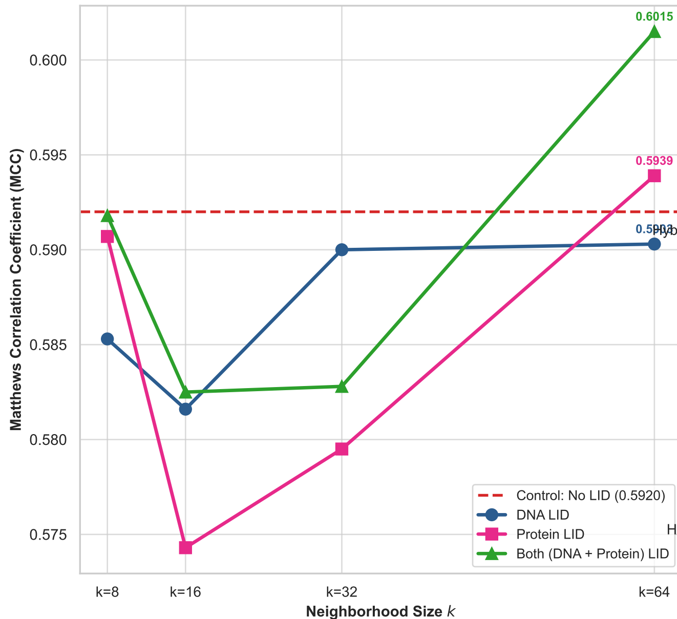
(A) LID Neighborhood Size k Ablation (ProteinGym)
