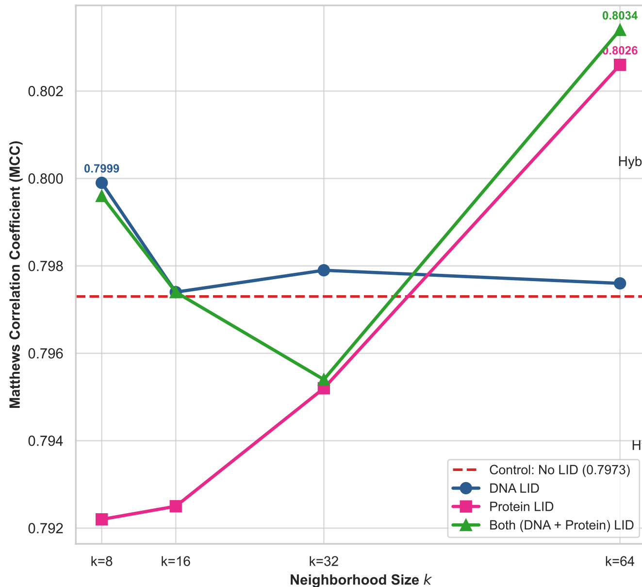
(A) LID Neighborhood Size k Ablation (Test)
