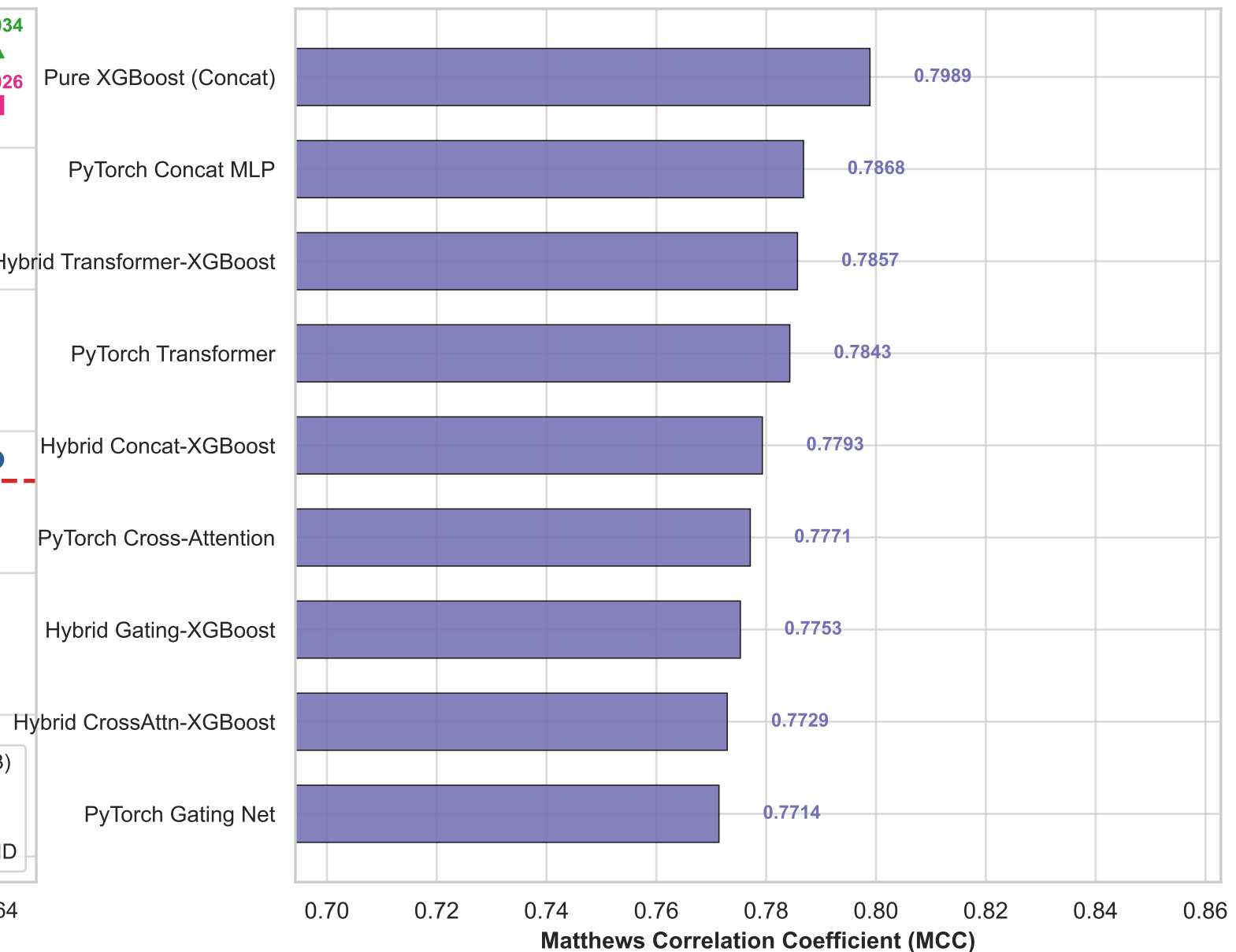
(B) Neural vs Hybrid vs Pure Architectures (Test - DNA k=32 )
