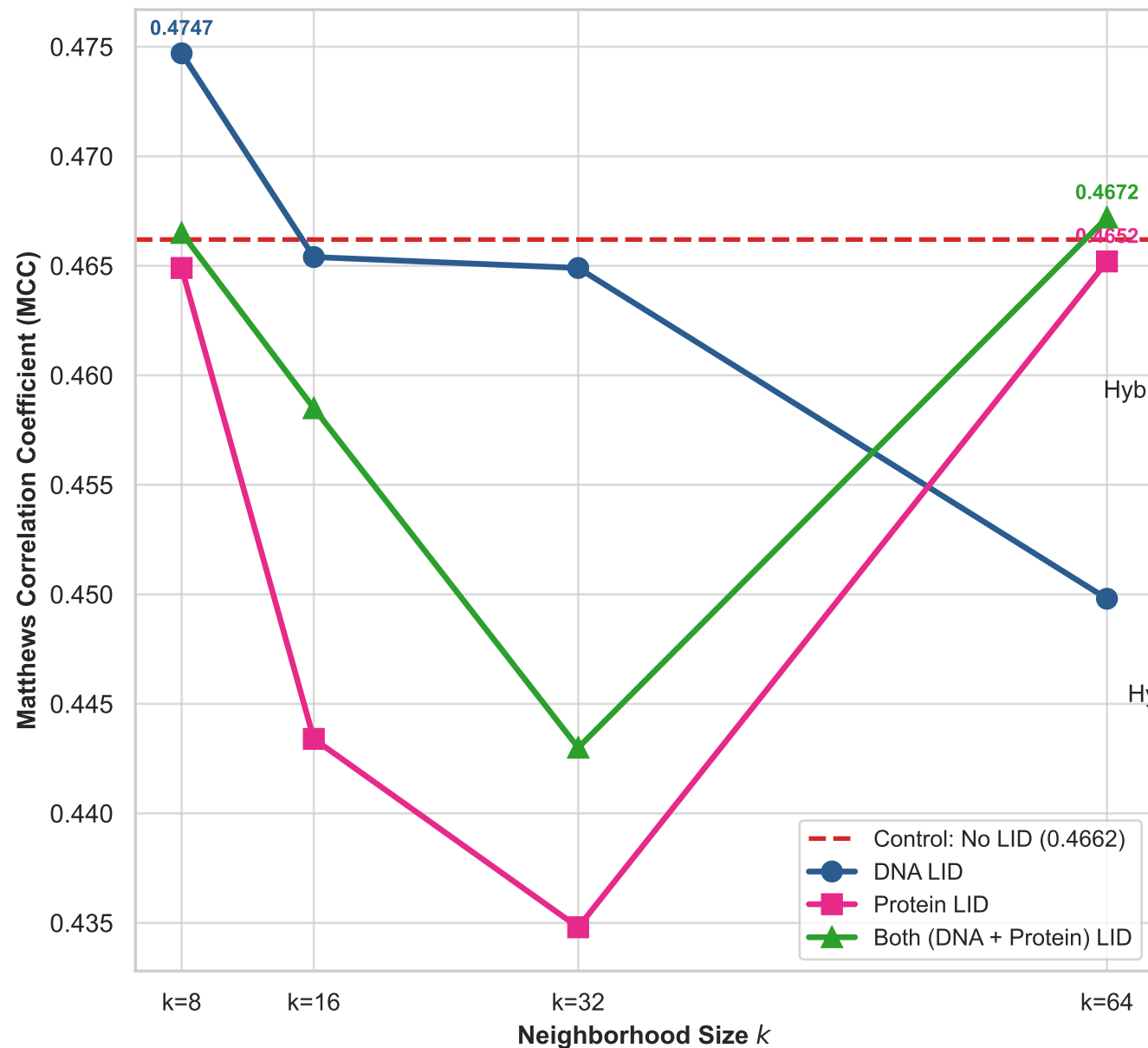
(A) LID Neighborhood Size k Ablation (UniProt)
