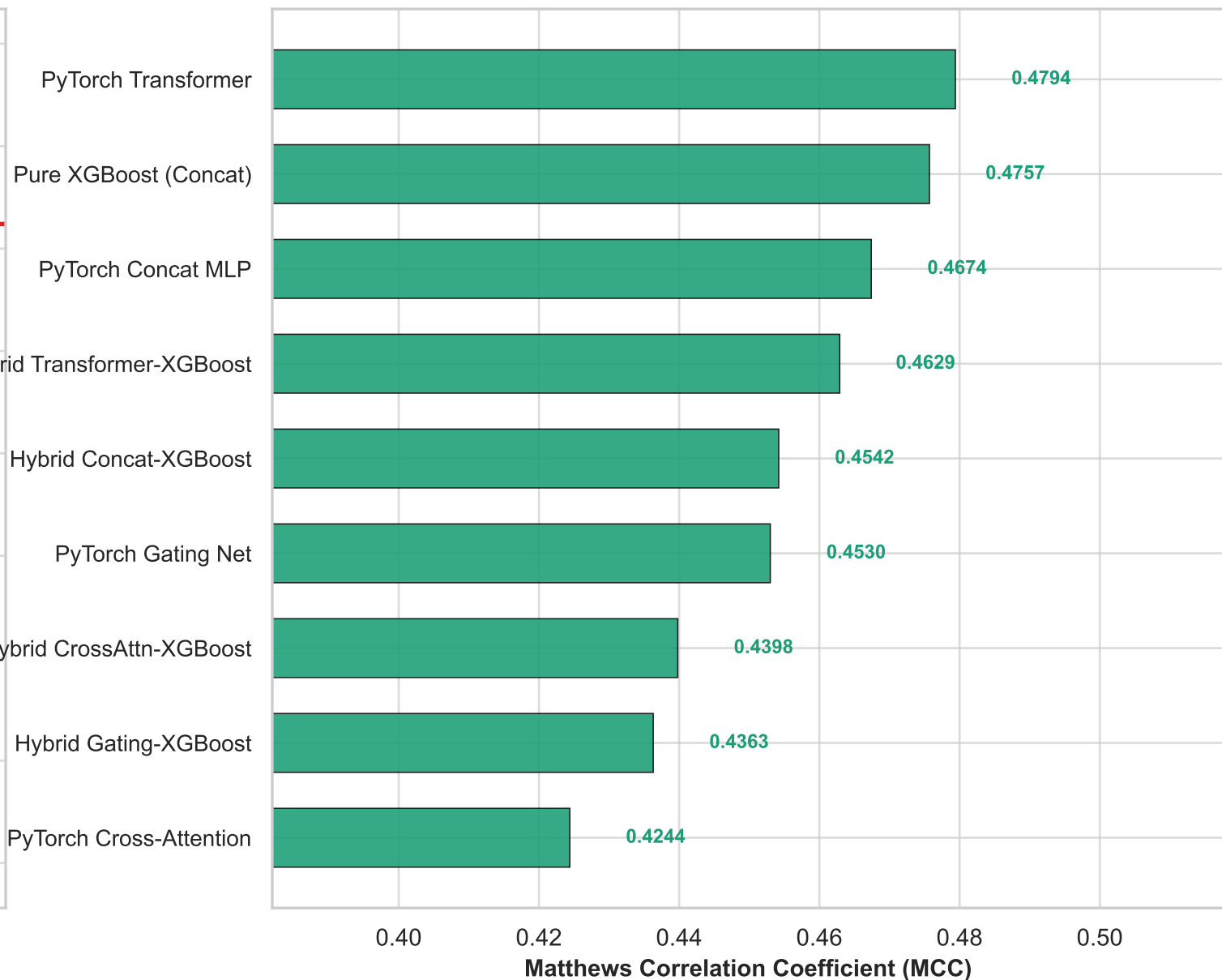
(B) Neural vs Hybrid vs Pure Architectures (UniProt - DNA k=32 )
