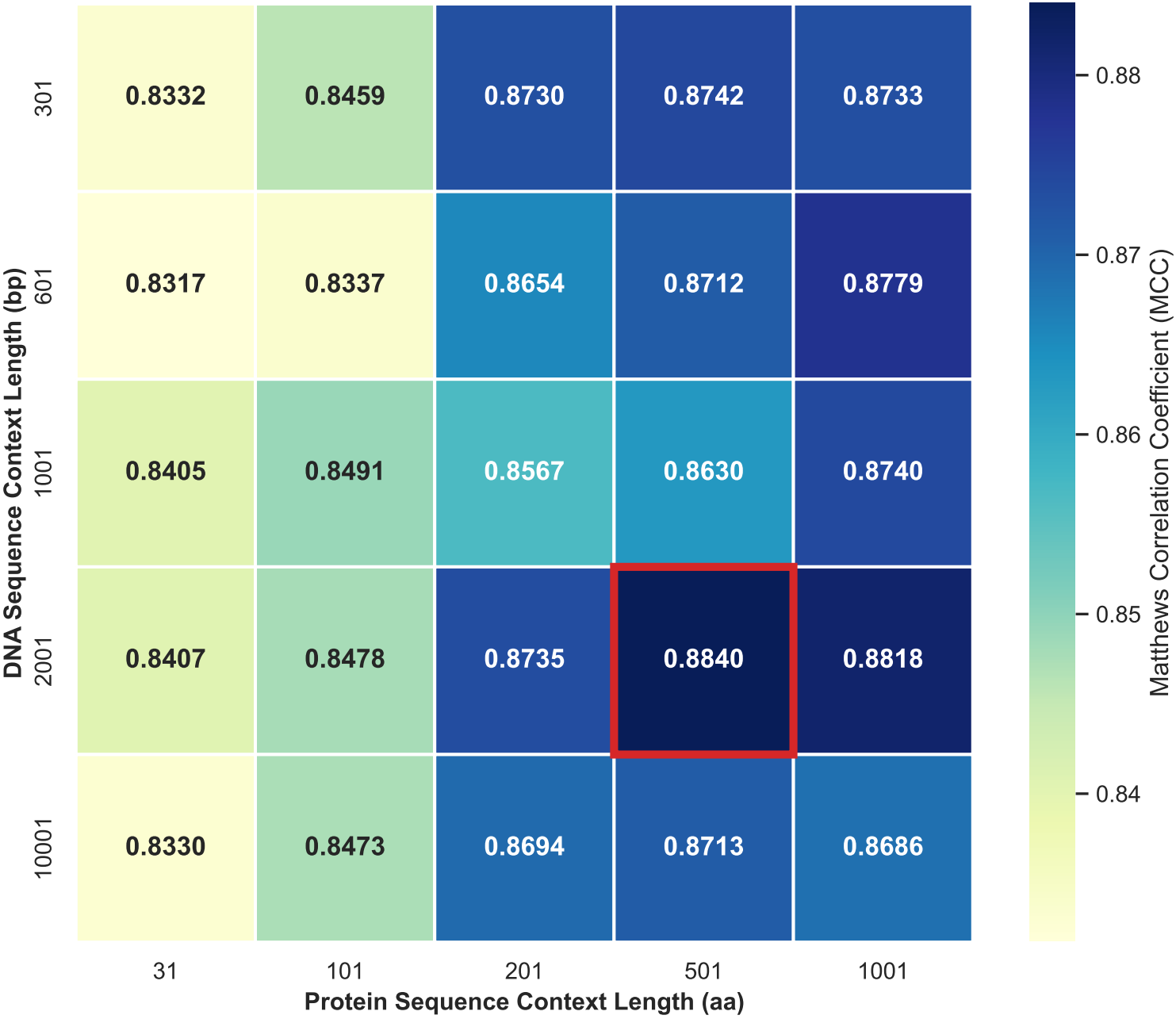
Sequence Context Length Grid - ClinVarHQ Optimal: DNA = 2001 bp, Protein = 501 aa (MCC = 0.8840, +6.09% vs shortest)
