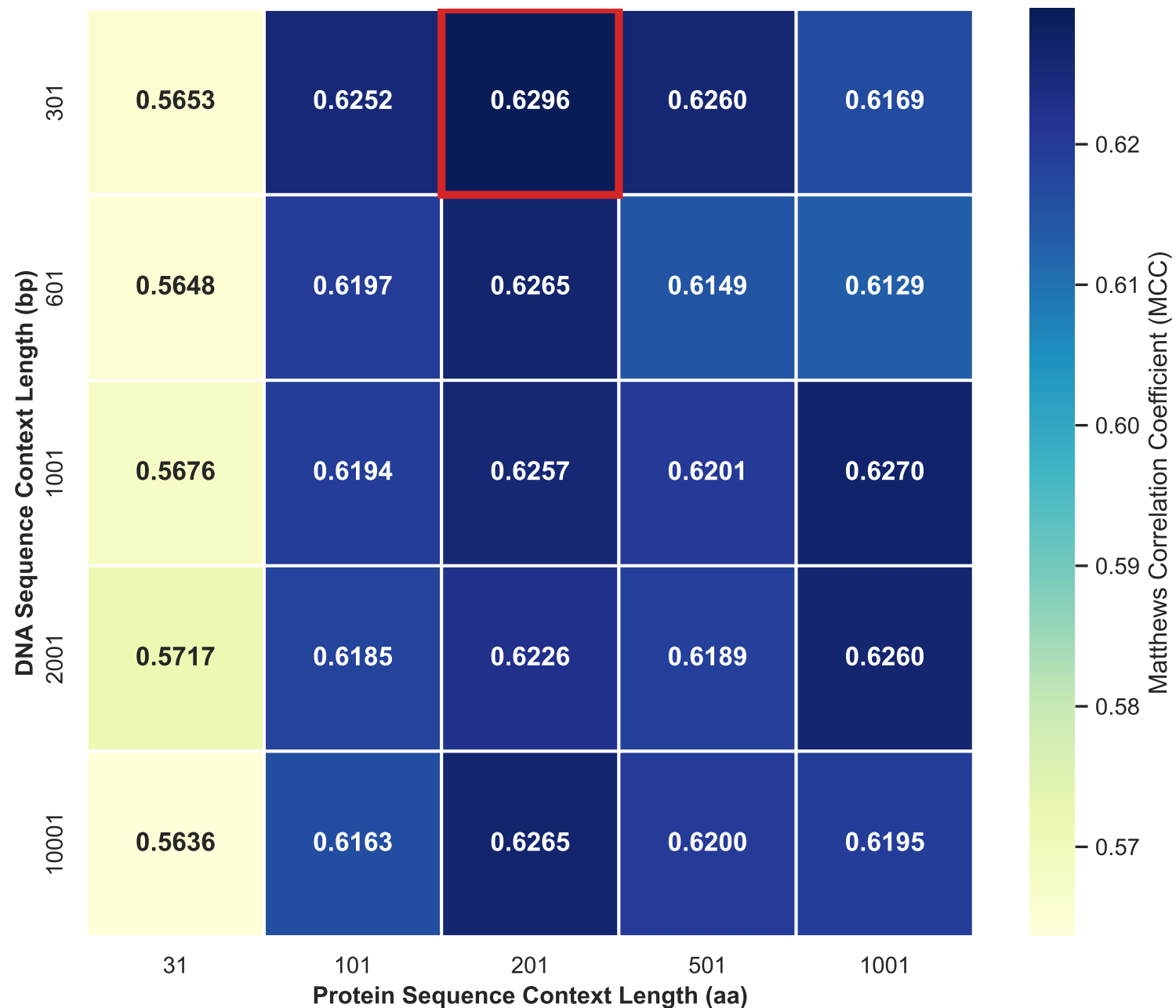
Sequence Context Length Grid - ProteinGym Optimal: DNA = 301 bp, Protein = 201 aa (MCC = 0.6296, +11.38% vs shortest)
