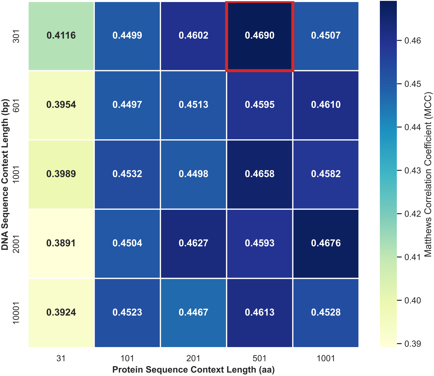
Sequence Context Length Grid - UniProt Optimal: DNA = 301 bp, Protein = 501 aa (MCC = 0.4690, +13.95% vs shortest)
