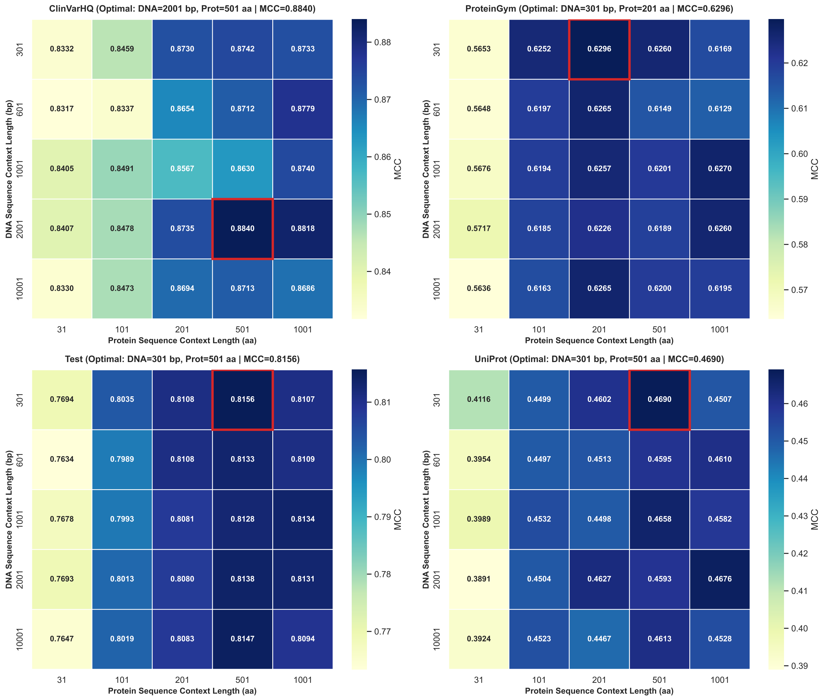
(A) Sequence Context Length Ablation across 4 Clinical Benchmarks (Averaged over 3-fold CV)
