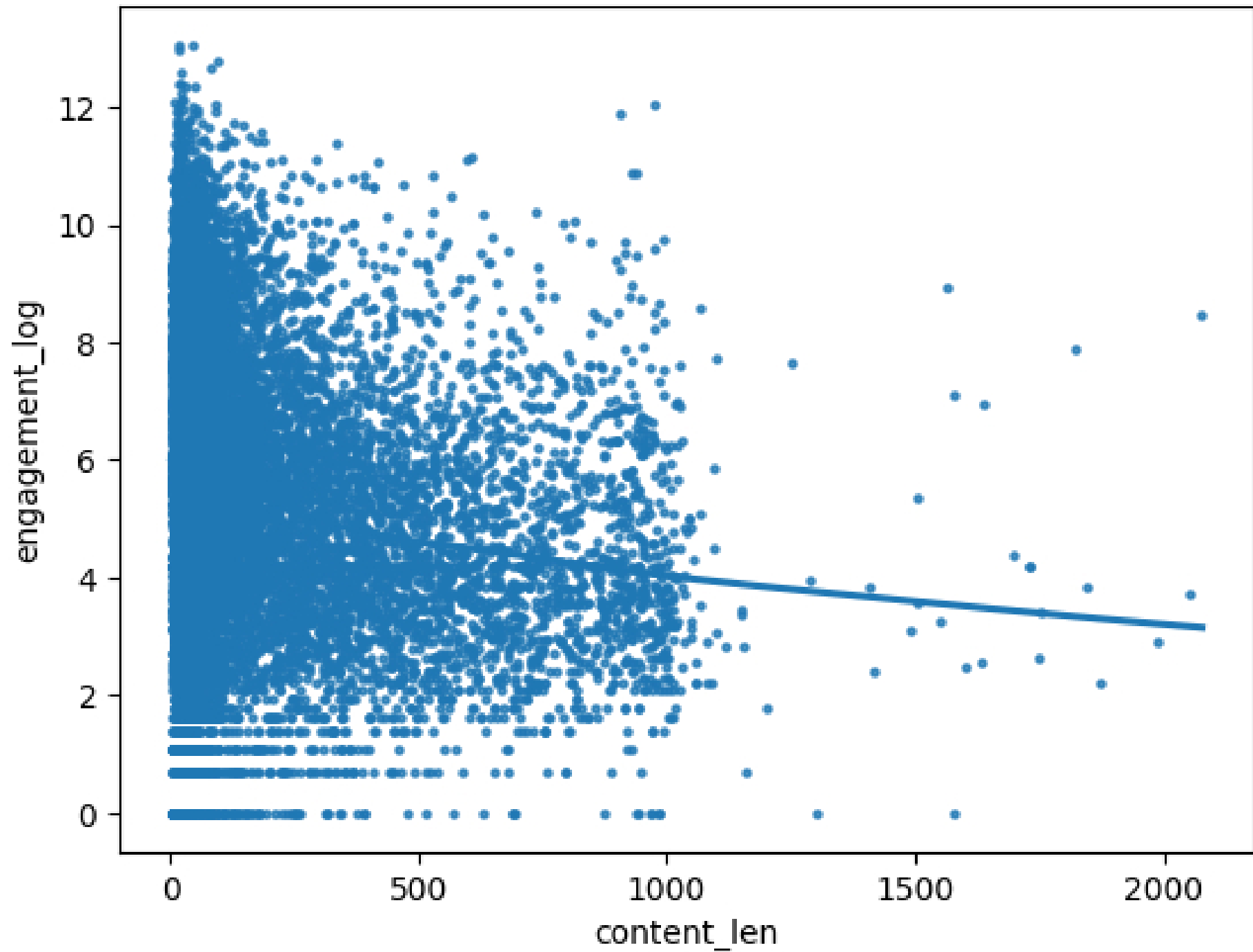
LOWESS
