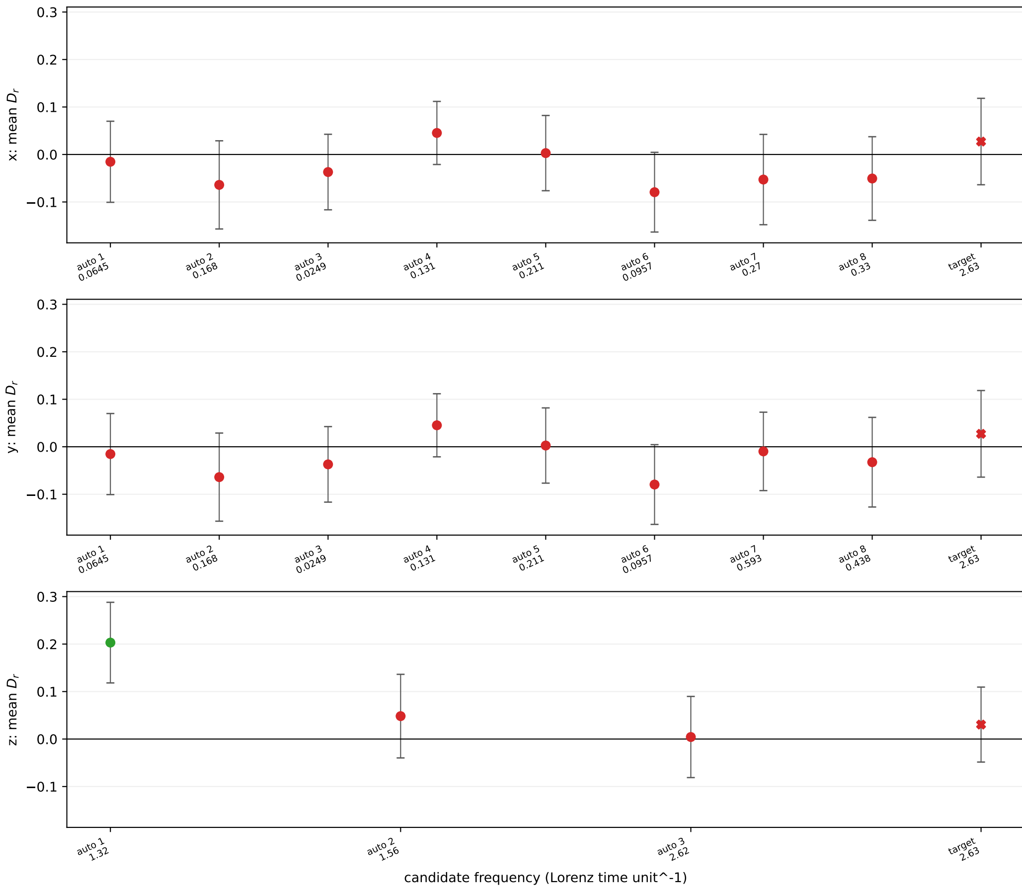
Test-seed peak/background significance circle: automatic peak; X: predefined target; green: coordinate-wise Holm significant
