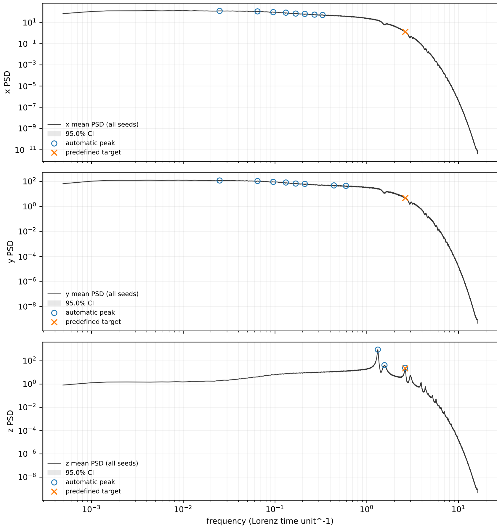
Coordinate-resolved natural spectra automatic peaks: 48 discovery seeds; significance: 48 test seeds; resolution=0.0004883
