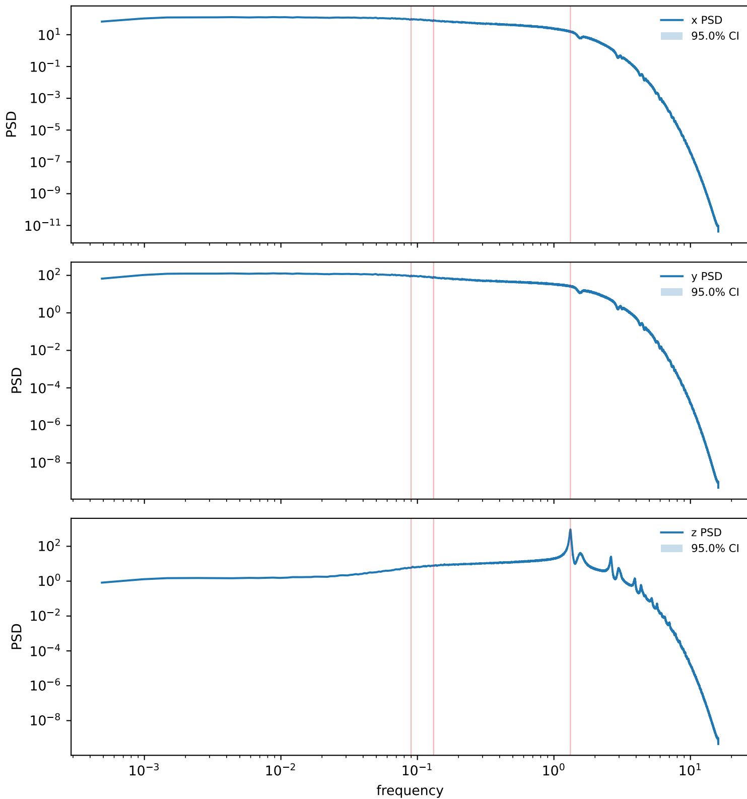
Natural spectrum resolution=0.0004883, Nyquist=16, Welch=32768, overlap=16384
