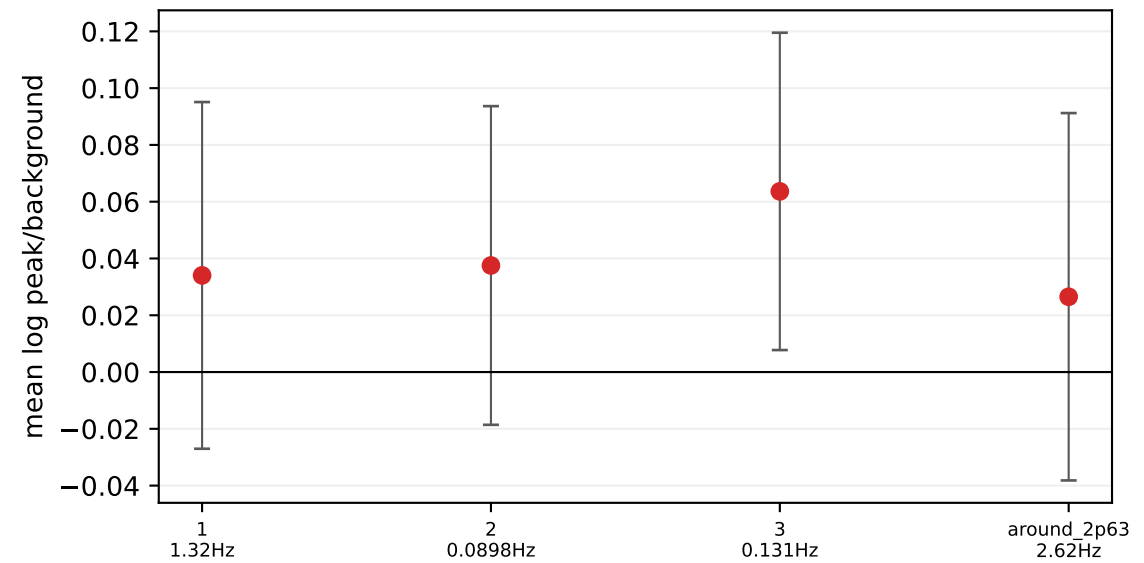
Natural spectrum peak significance green: Holm-adjusted significant; red: not significant
