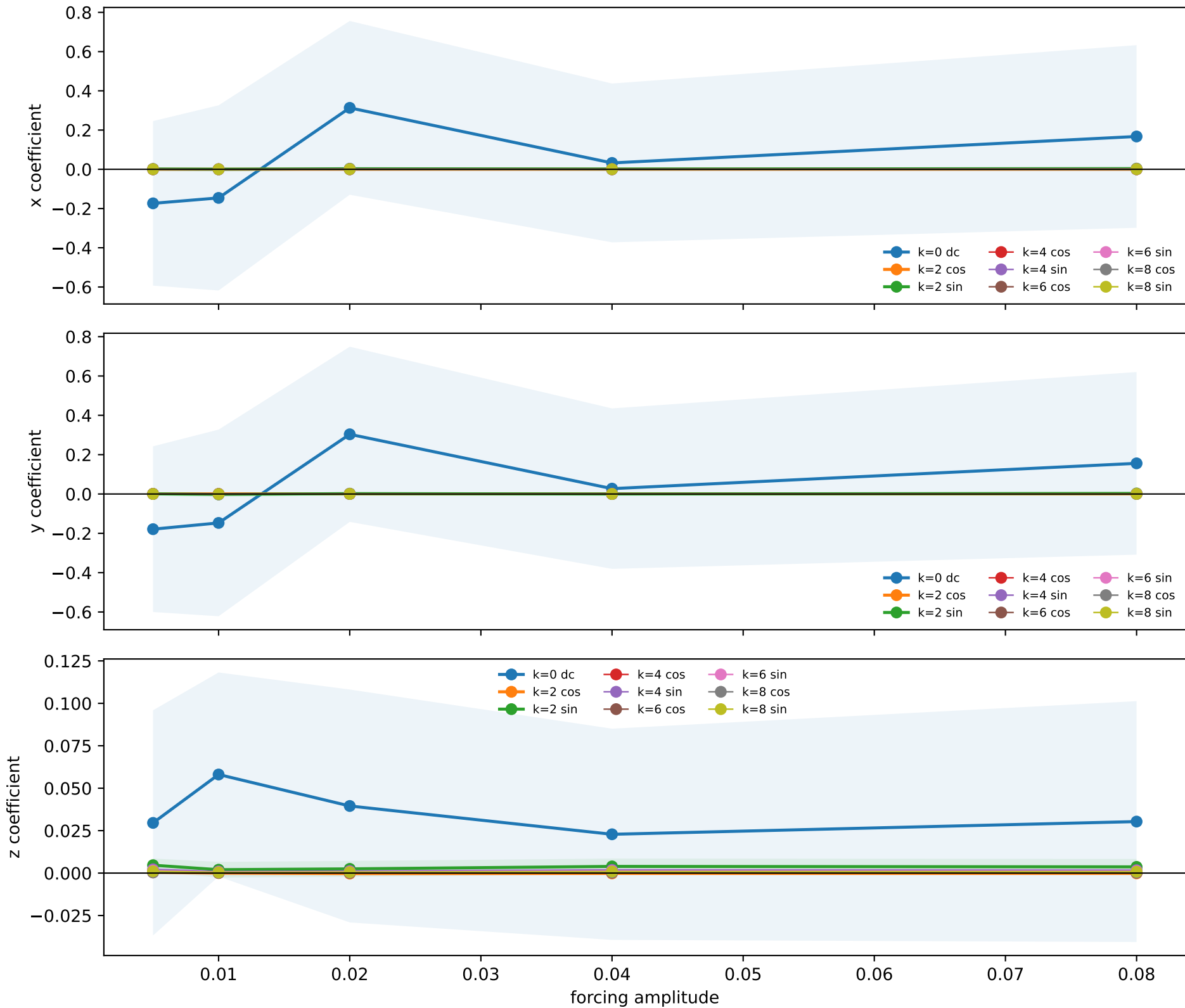
\omega=32.9591 , forcing direction=2, even response signed FFT/Fourier coefficient seed mean and 95.0% Student-t CI
