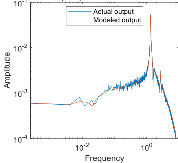
Output spectrum on z-direction
