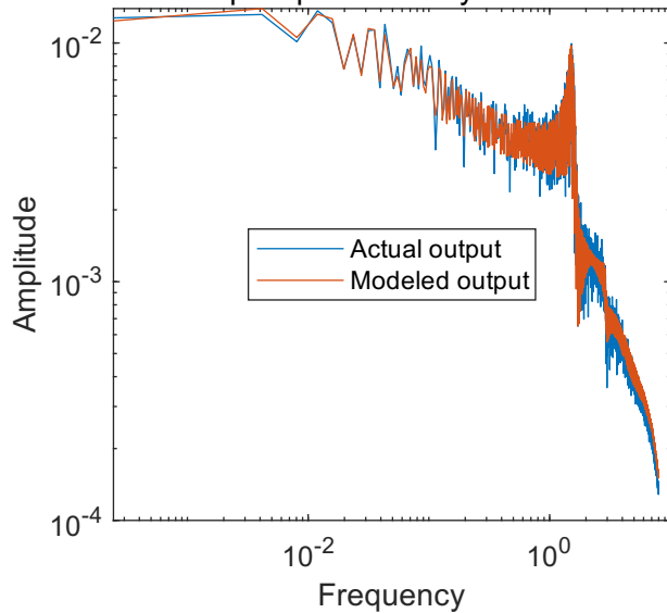
Output spectrum on y-direction
