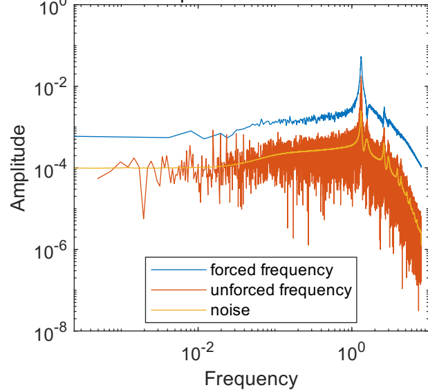
Response on z-direction
