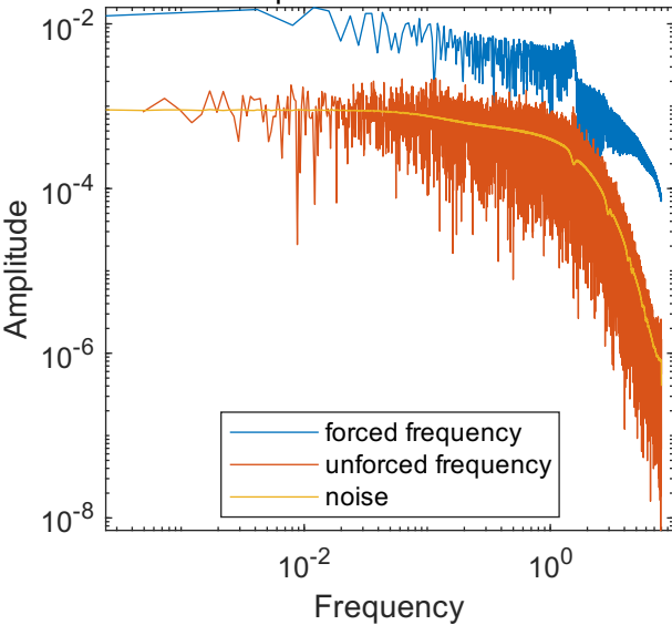
Response on x-direction
