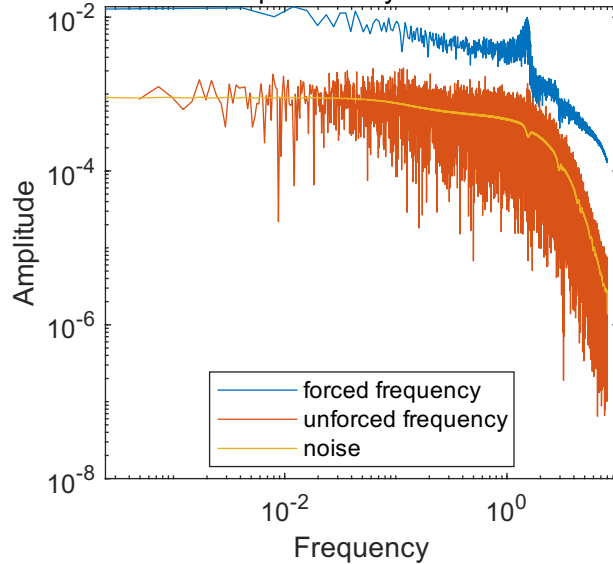
Response on y-direction
