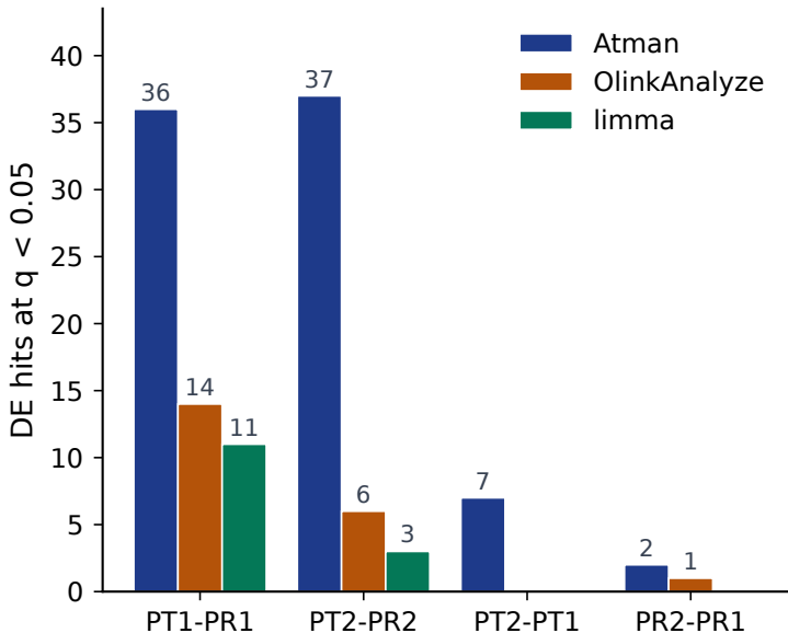
Per-tool DE yield across four Dube contrasts
