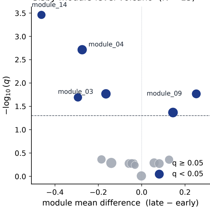
Gisby module-level volcano (K = 15)
