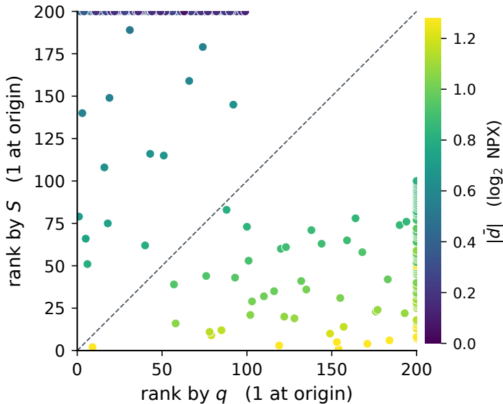
Dube PT1-PR1: q -rank vs S -rank
