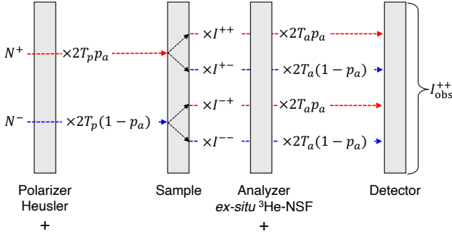
FIG. 8. Schematic diagram of the spin-dependent neutron intensities in the present experimental setup when the Heusler polarizer and the ^3\text{He} -NSF are both set to select up-spin (+) neutrons. The red and blue lines indicate the paths of the up neutrons ( N^+ ) and down neutrons ( N^- ), respectively. The observed intensity, I_{\text{obs}}^{++} , is obtained as the sum of the contributions from the four spin-scattering channels.
