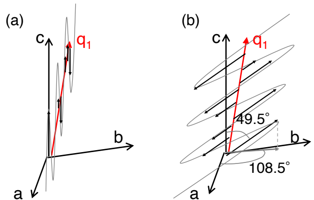
FIG. 8. Schematic illustrations of the sinusoidal magnetic structures. (a) the c -axis-parallel sinusoidal model and (b) the oblique sinusoidal model. The red arrow indicates the magnetic propagation vector \mathbf{q}_1 , and the black arrows represent the modulated magnetic moments. In the oblique sinusoidal model, the moment direction is specified by the polar angles measured from the c -axis and azimuthal angles measured from the a -axis, denoted as \theta and \phi , respectively.
