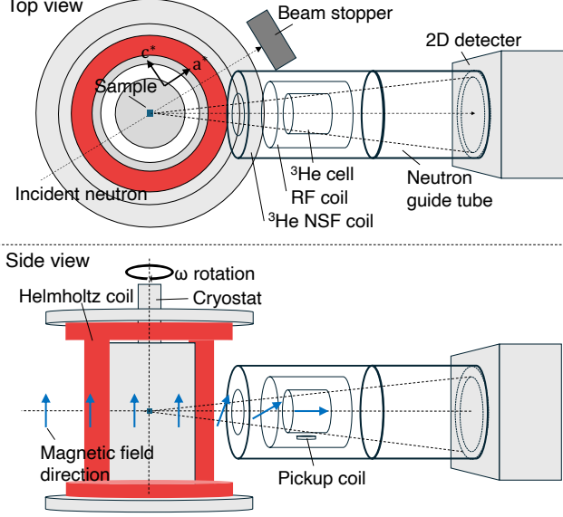
FIG. 2. Schematic illustration of a polarization analysis method enabling broad coverage of reciprocal lattice points in three-dimensional reciprocal space.
