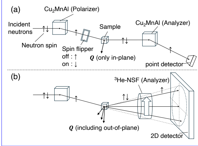
FIG. 1. Schematic illustrations comparing neutron polarization analysis techniques. (a) Conventional setup using a \text{Cu}_2\text{MnAl} crystal for both polarizer and analyzer, where only in-plane scattered neutrons are detected by a point detector. (b) Polarization analysis setup using a ^3\text{He} -NSF combined with a two-dimensional detector, enabling detection of both in-plane and out-of-plane scattered neutrons.
