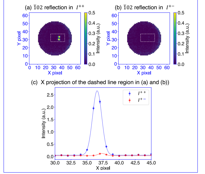
FIG. 4. (a) Non-spin-flip intensity ( I^{++} ) and (b) spin-flip intensity ( I^{+-} ) maps, showing only the region covered by the ^3\text{He} cell. A clear difference in the intensity of the \bar{1}02 nuclear Bragg peak is observed depending on the direction of the ^3\text{He} polarization. (c) Line profile along the (x) direction obtained by integrating the intensity within the dashed regions in (a) and (b).
