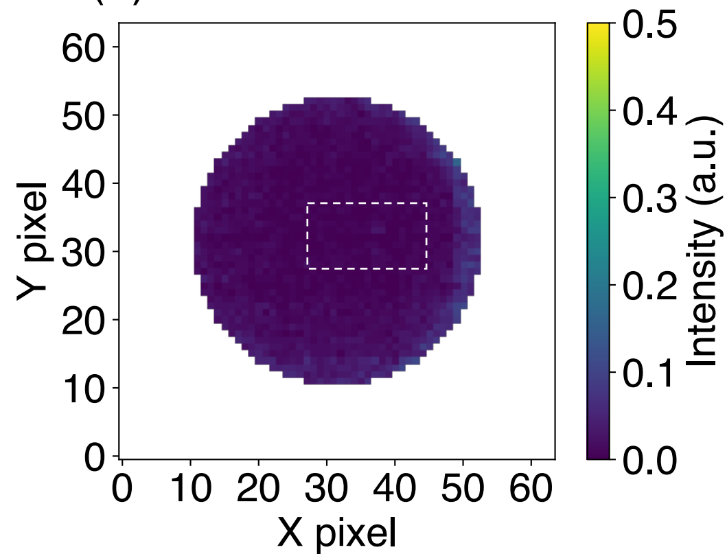
(b) \bar{1}02 reflection in I^{+-}
