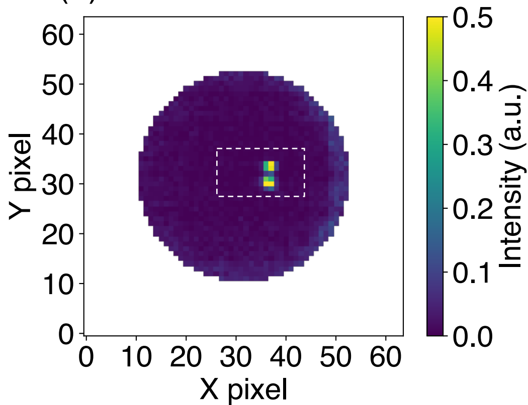
(a) \bar{1}02 reflection in I^{++}
