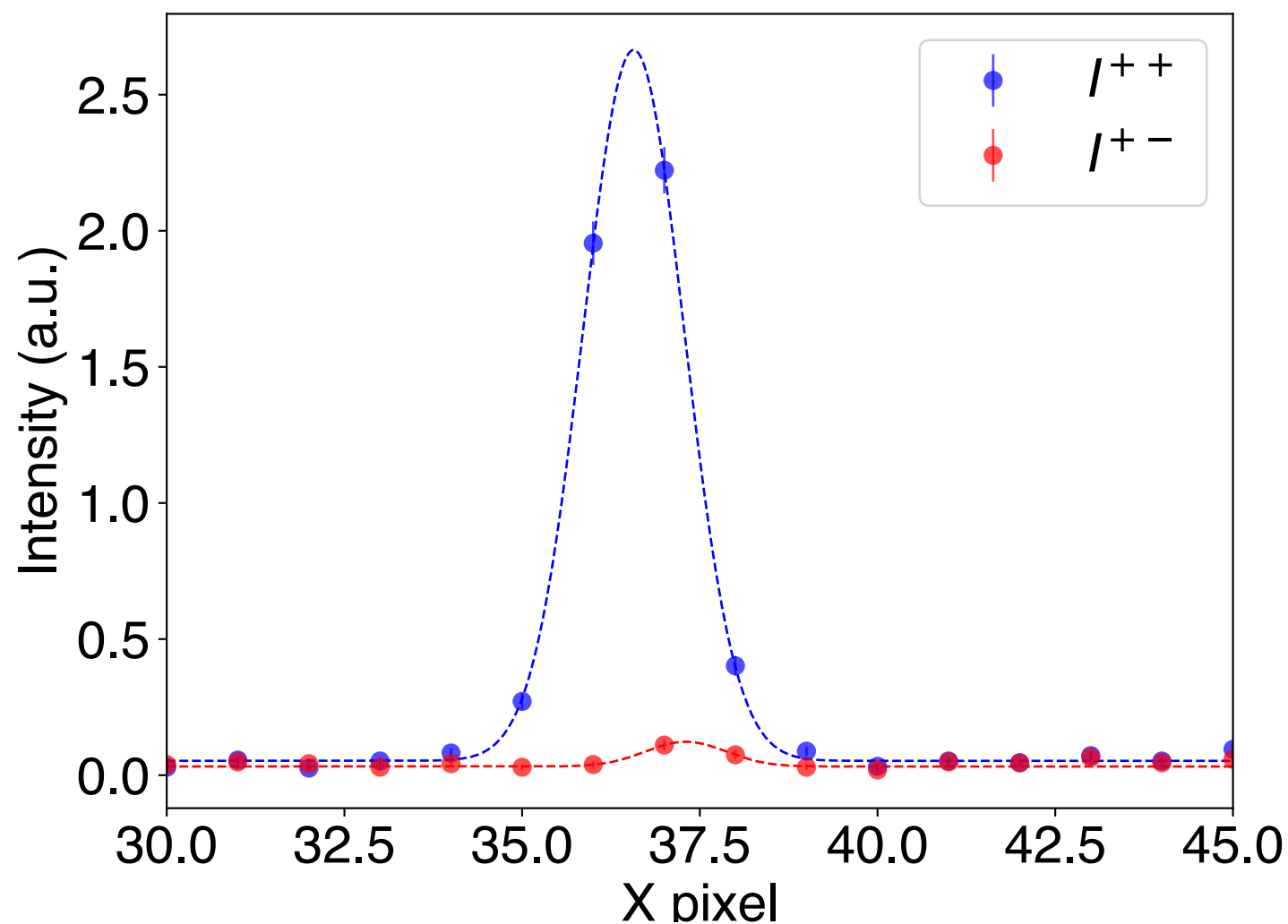
(c) X projection of the dashed line region in (a) and (b)
