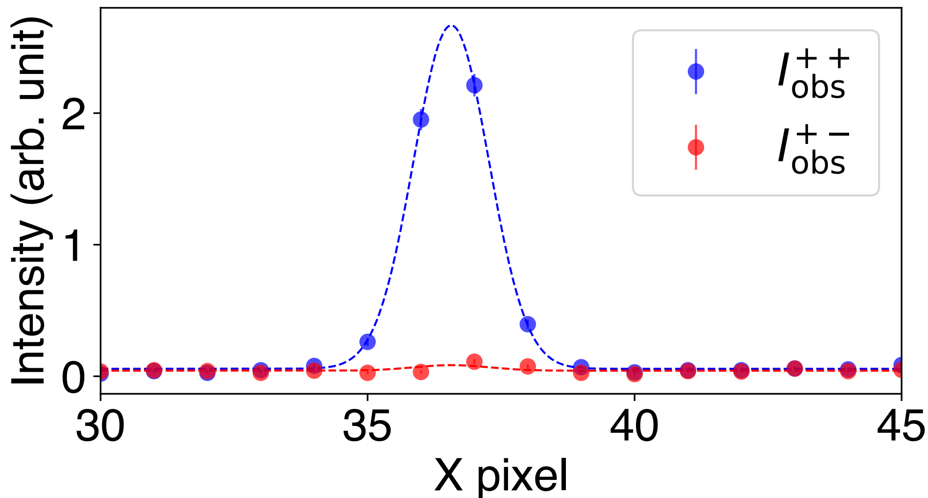
(c) X projection of the dashed line region in (a) and (b)
