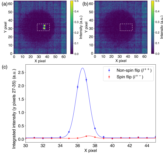
FIG. 3. (a) Non-spin-flip ( I^{++} ) and (b) spin-flip ( I^{+-} ) scattering intensity maps. A clear difference in the nuclear Bragg peak intensity is observed upon flipping the ^3\text{He} polarization. The dashed boxes indicate the integration region. (c) Line profile along the x direction obtained by integrating the intensity within the dashed region in (a) and (b).
