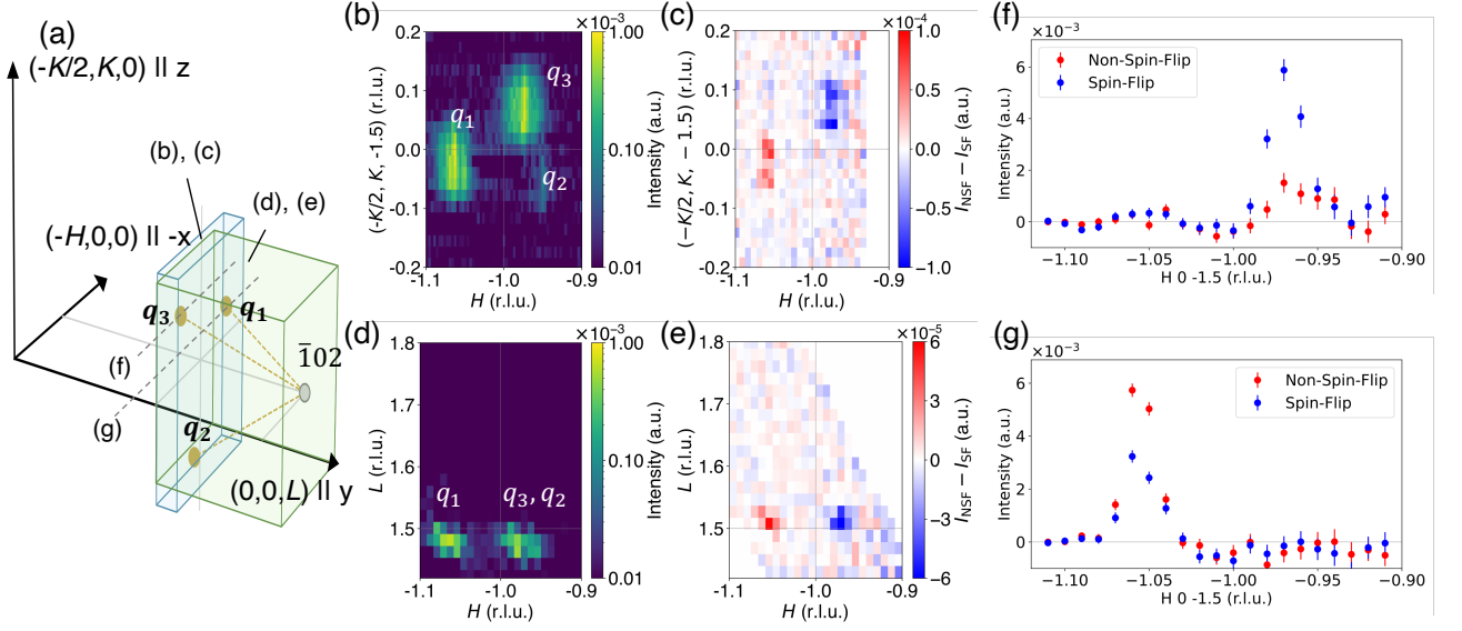
FIG. 6. (a) Schematic illustration of the reciprocal-space region measured in the present experiment. The translucent volumes labeled (b), (c) and (d), (e) indicate the regions integrated along the L direction and the (-K/2, K, 0) direction, respectively. The dashed lines along the -H direction through q_3 and q_1 indicate the line cuts shown in panels (f) and (g), respectively. (b), (d) Unpolarized neutron intensity maps in the (H, K/2, -1.5) and (H, 0, L) planes, respectively. (c), (e) Corresponding polarization-analysis maps obtained from the difference between the non-spin-flip and spin-flip intensities, I^{++} - I^{+-} . (f), (g) Line profiles of the non-spin-flip and spin-flip intensities at q_3 and q_1 , respectively.
