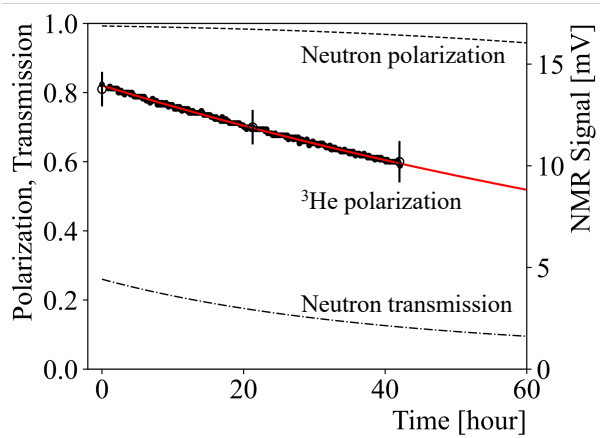
FIG. 4. Time dependence of the ^3\text{He} polarization, neutron polarization, and neutron transmission. The open circles show the ^3\text{He} polarization obtained from the intensity of the (102) nuclear Bragg peak, while the closed circles show the NMR signal of ^3\text{He} . The red line represents the fitting result using an exponential decay function. The dashed line indicates the calculated neutron polarization, and the dot-dashed line indicates the calculated neutron transmission.
