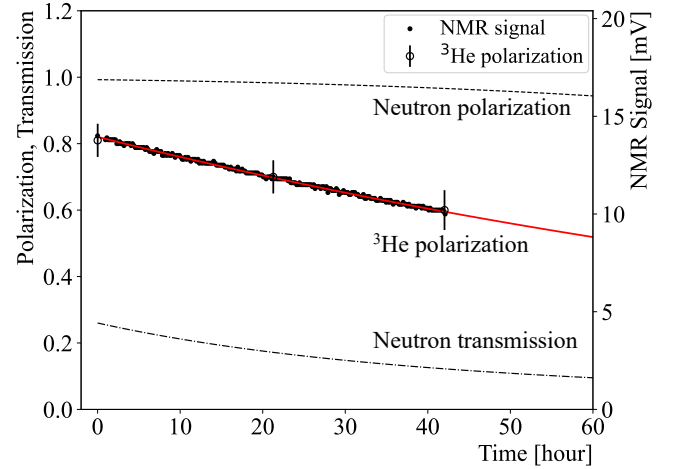
FIG. 5. Time dependence of the ^3\text{He} polarization, neutron polarization, and neutron transmission. The open circles show the ^3\text{He} polarization determined from the intensity of the 102 nuclear reflection, while the closed circles show the ^3\text{He} NMR signal. The red line represents the fitting result using an exponential decay function. The dashed and dot-dashed lines indicate the calculated neutron polarization and transmission, respectively, obtained from the ^3\text{He} polarization.
