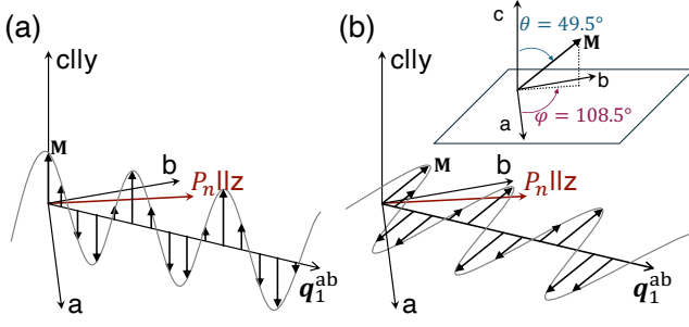
FIG. 8. Schematic illustrations of the sinusoidal magnetic structures. (a) the c -axis-parallel sinusoidal model and (b) the oblique sinusoidal model. The \mathbf{q}_1^{ab} vector is the projection of the magnetic propagation vector \mathbf{q}_1 onto the ab plane. The P_n vector is the neutron polarization direction, which is parallel to the z axis in Fig. 7(a). Inset of the panel (b) shows the definition of the polar angle \theta and azimuthal angle \phi . In the oblique sinusoidal model, the magnetic moment direction \mathbf{M} is specified by \theta = 49.5^\circ and \phi = 108.5^\circ .
