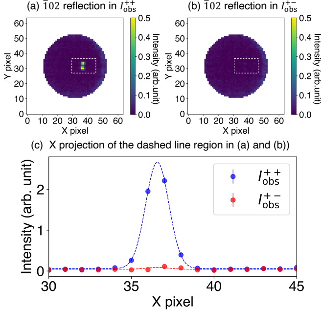
FIG. 4. (a) Observed non-spin-flip ( I_{\text{obs}}^{++} ) and (b) spin-flip ( I_{\text{obs}}^{+-} ) intensity maps, showing only the analyzing region. (c) Line profile along the X direction, obtained by integrating the intensity within the rectangular regions indicated by the dashed lines in (a) and (b).
