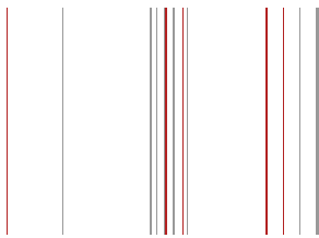
Genes in Region (red = nearest to hubs)
