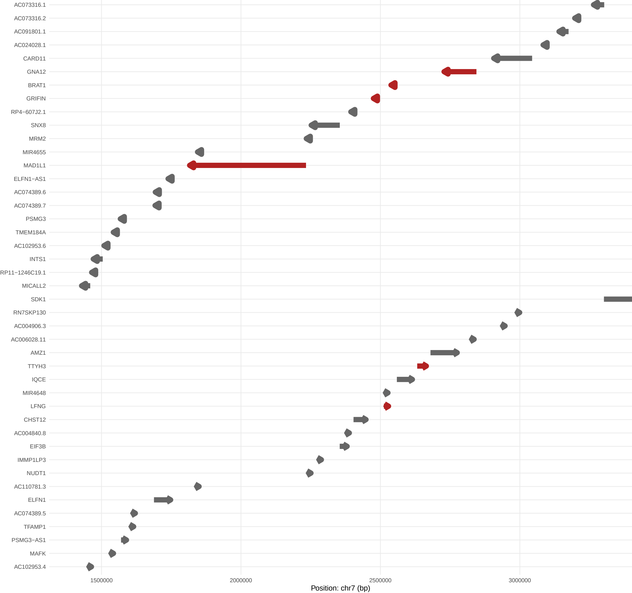
Genes in Region (red = nearest to hubs)
