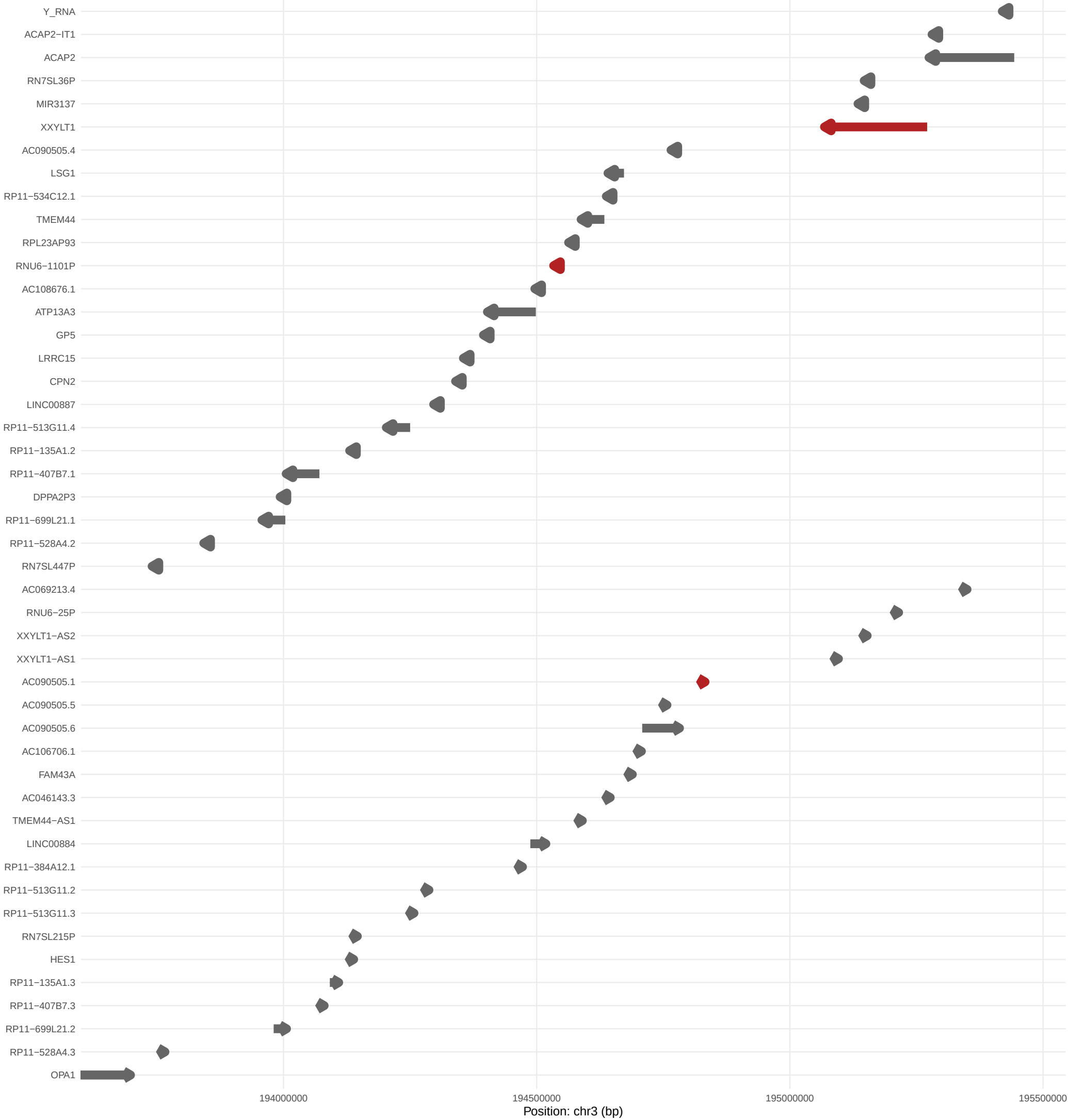
Genes in Region (red = nearest to hubs)
