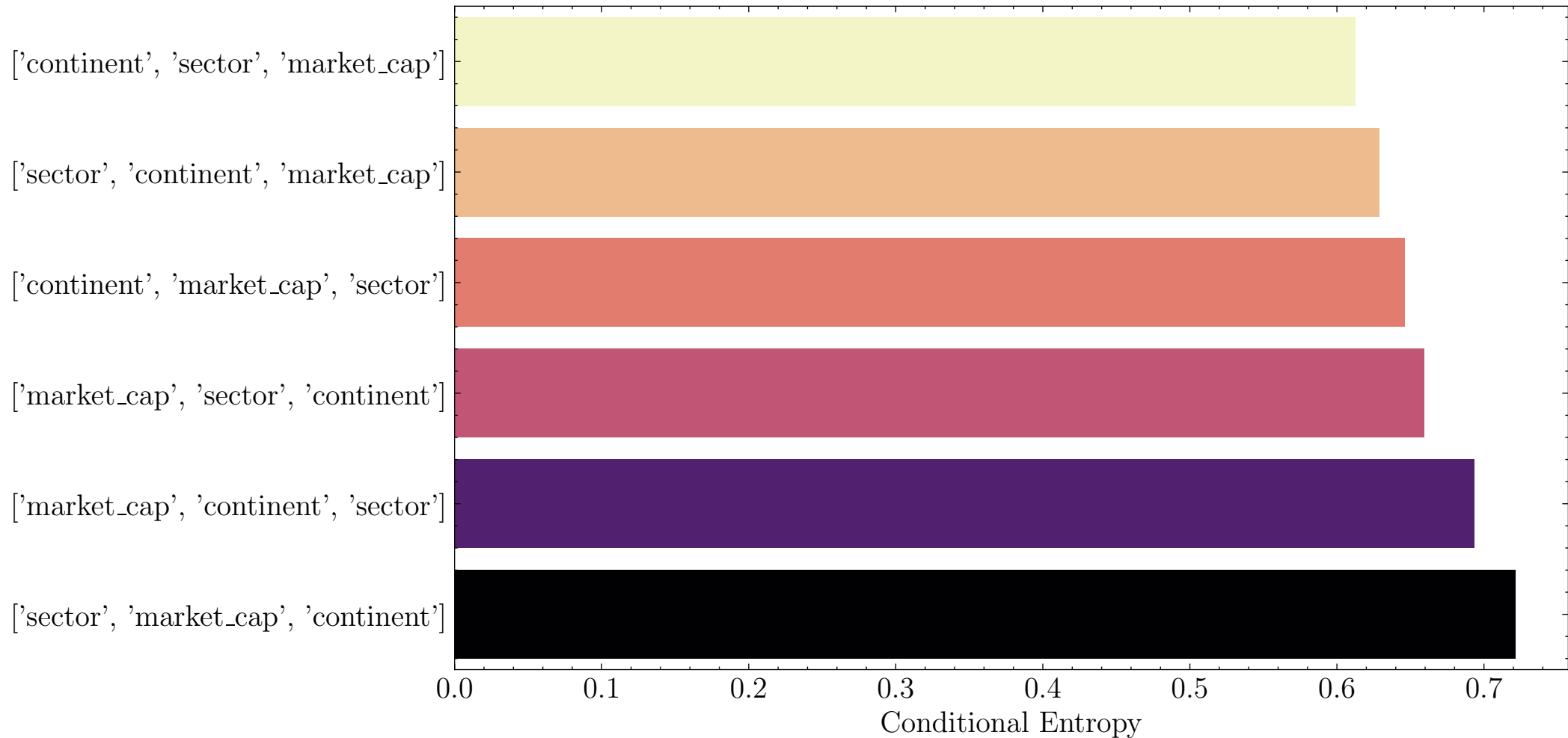
Entropy Reduction from Context Permutations
