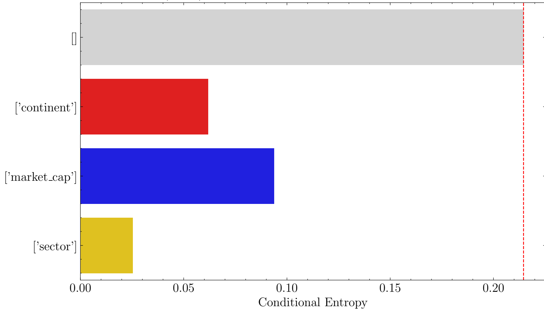
(Qwen) Entropy Reduction from Context Combinations
