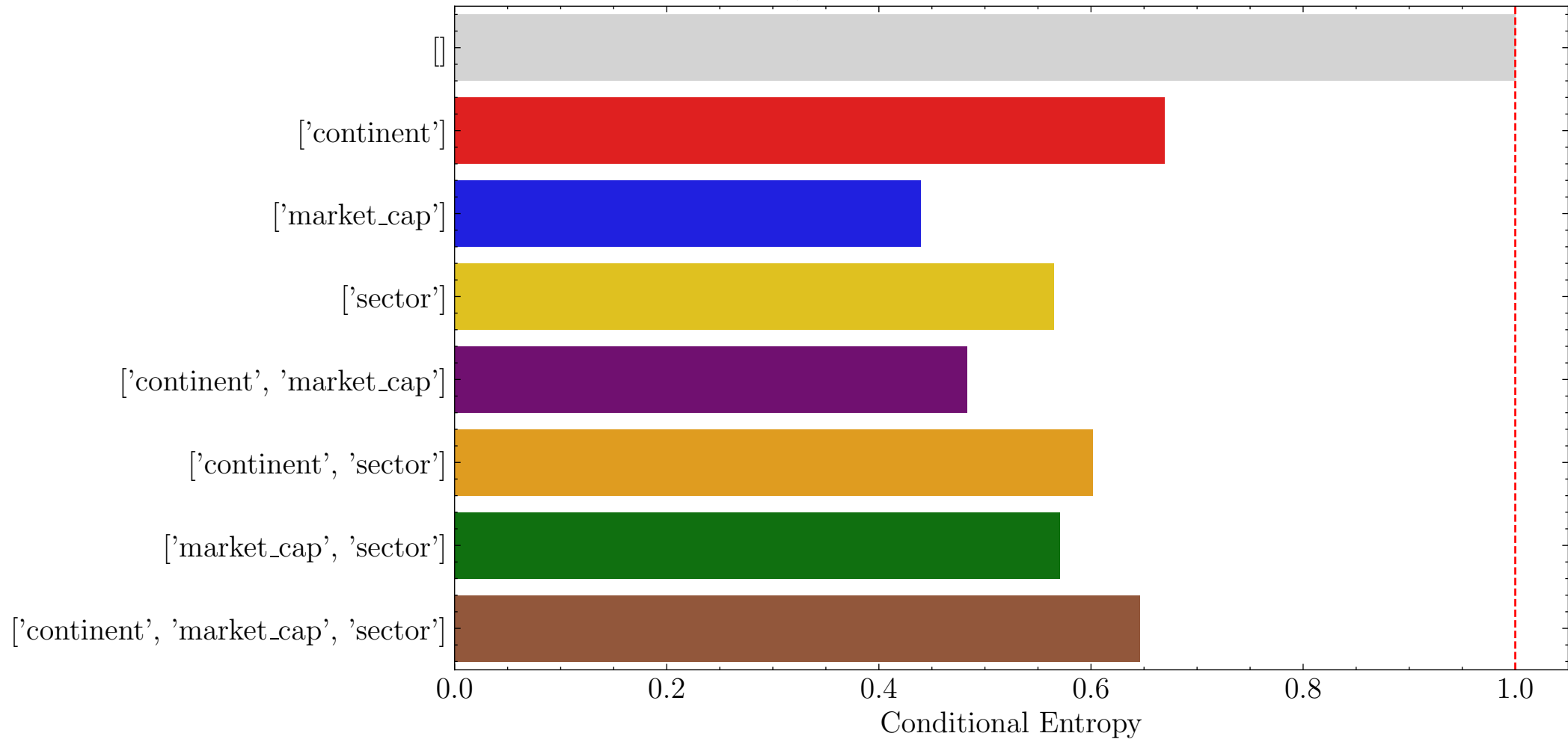
Entropy Reduction from Context Combinations
