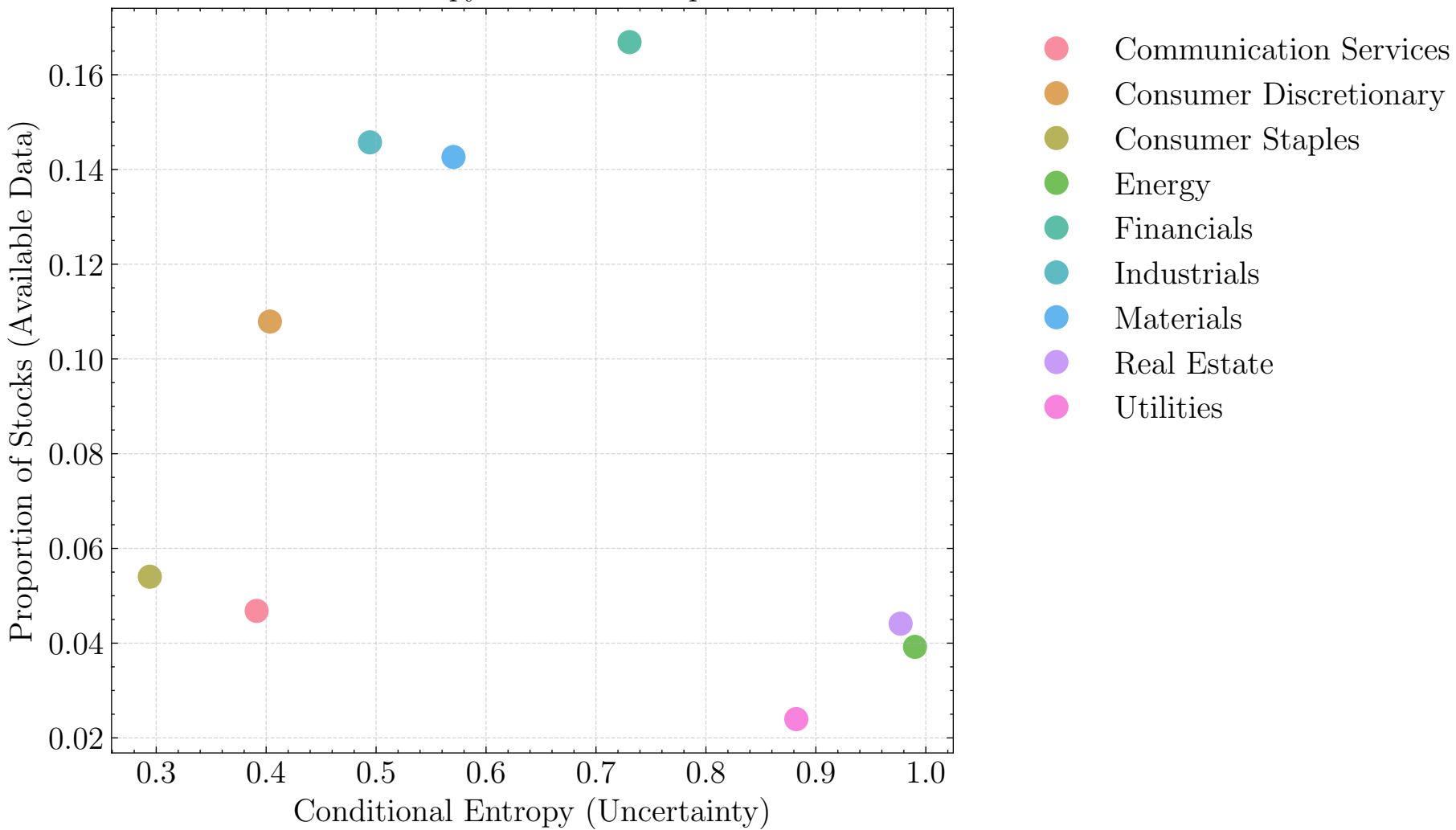
Model Entropy vs. Sector Proportion
