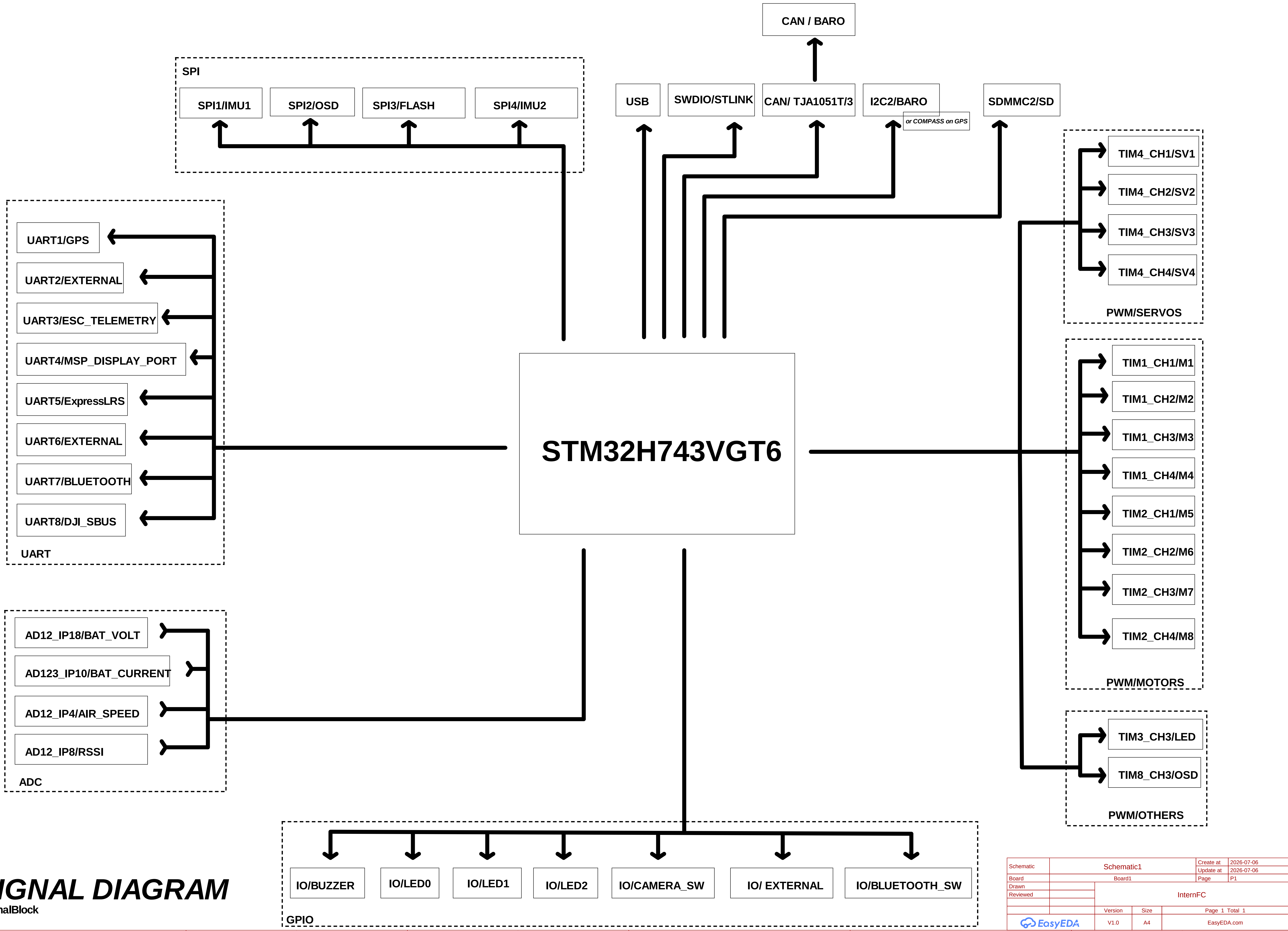
STM32H743Pro Wiring diagram
