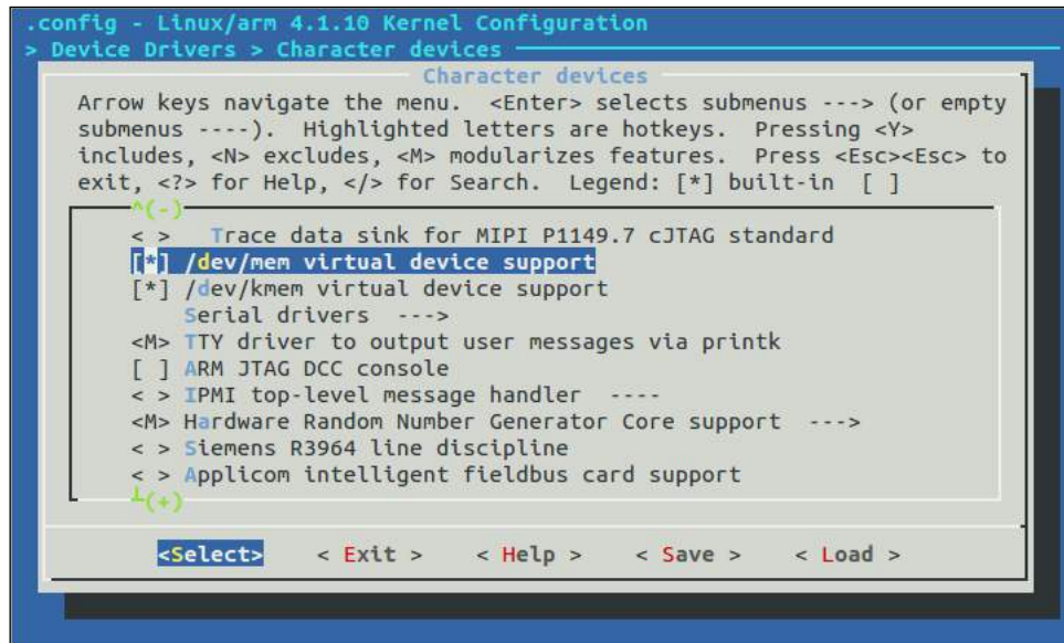
Kernel configuration using menuconfig
