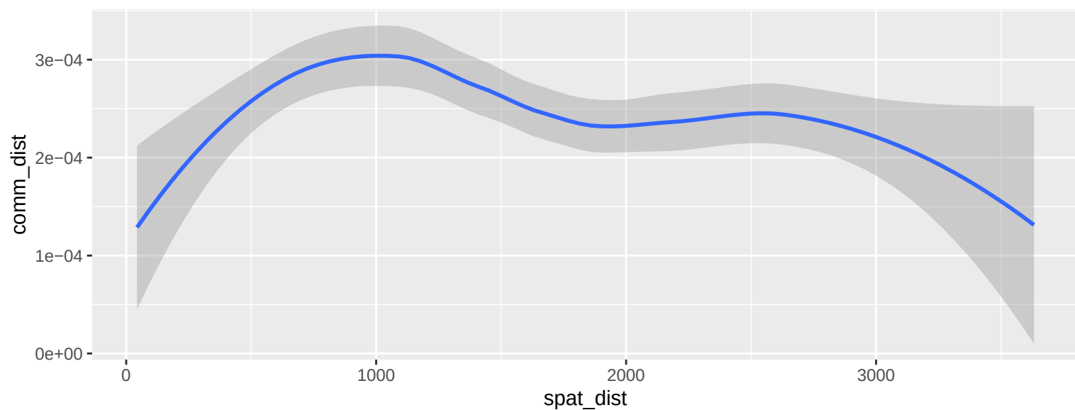
Spatial vs ANI distance: GPB_bin_000063
