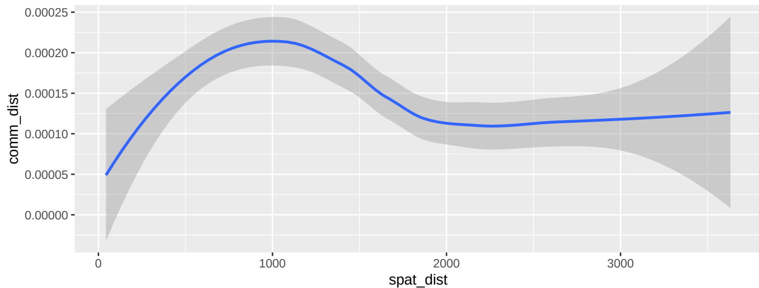
Spatial vs ANI distance: GPB_bin_000047
