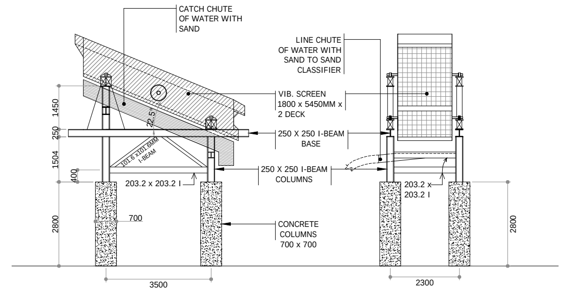
SET-UP OF VIBRATING SCREEN 1:100
