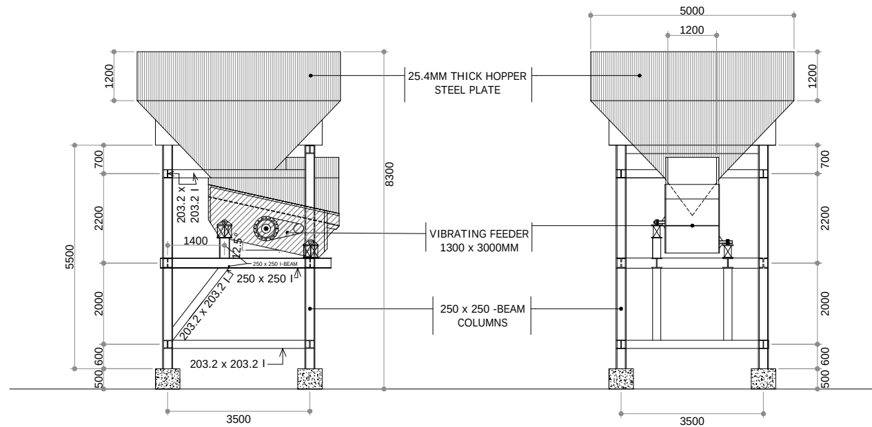
SET-UP OF VIBRATING FEEDER 1:100
