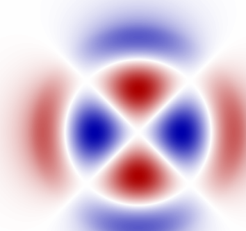
LP_{22}
