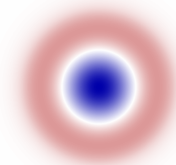
LP_{02}
