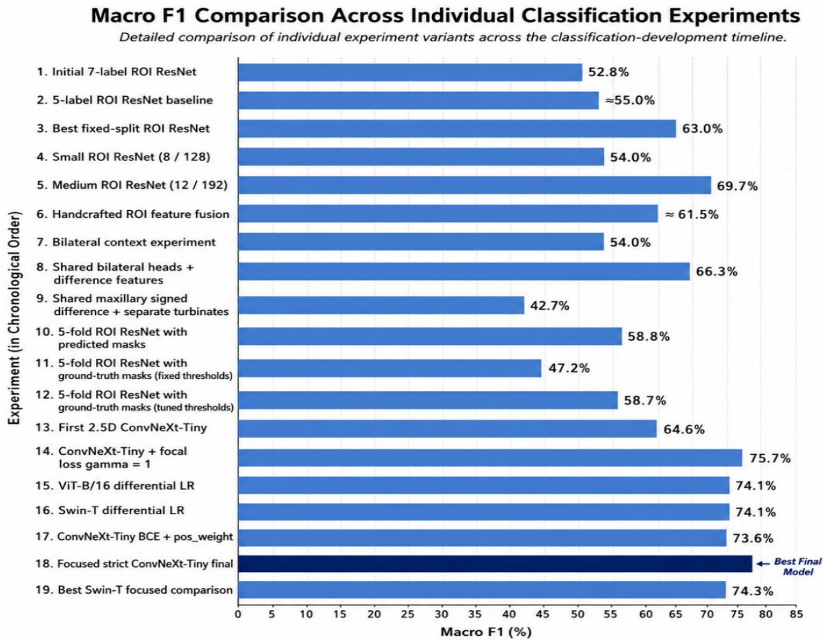
Figure 4.8: Macro F1 comparison across experiments.
