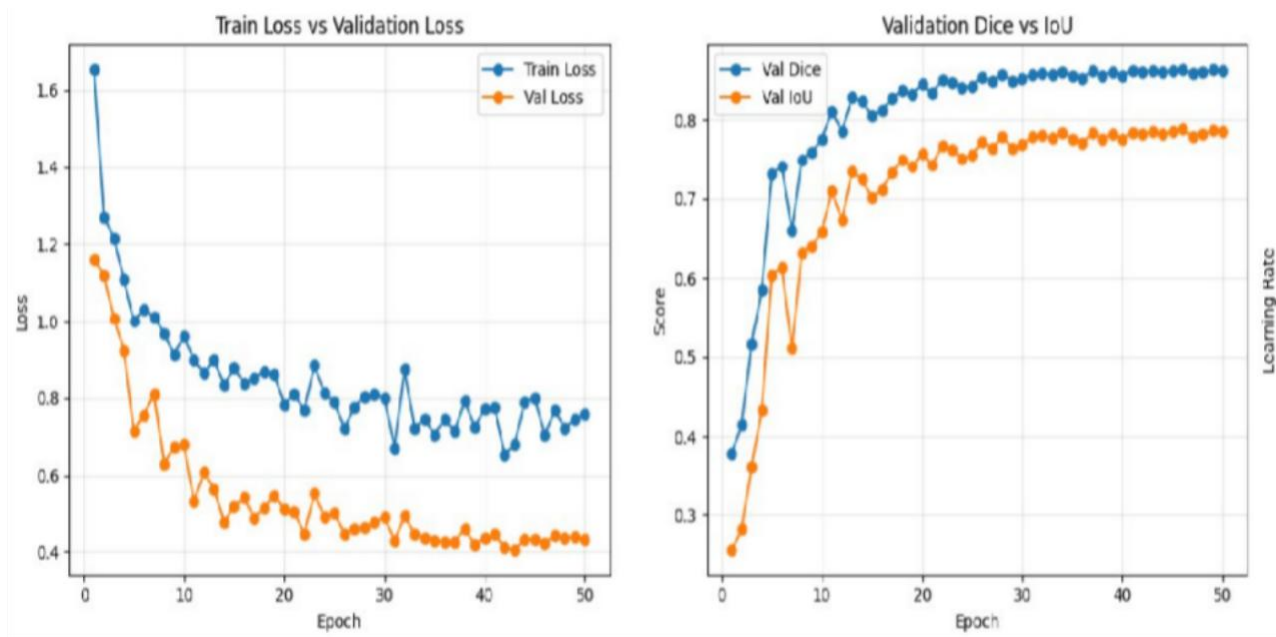
Figure 5.1: SwinUNETR training and validation curves
