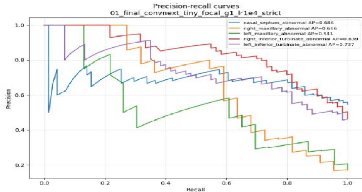
Figure 5.7: Precision-Recall curves for the final ConvNeXt-Tiny model
