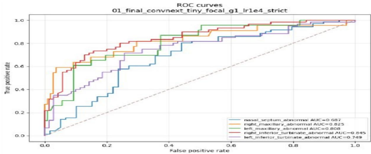
Figure 5.6: ROC curves for the final ConvNeXt-Tiny model
