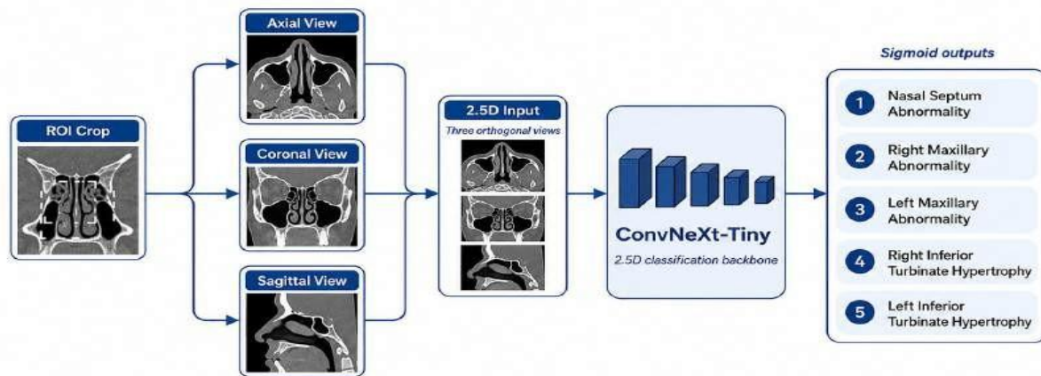
Figure 2.3: Simplified ConvNeXt-Tiny classification concept
