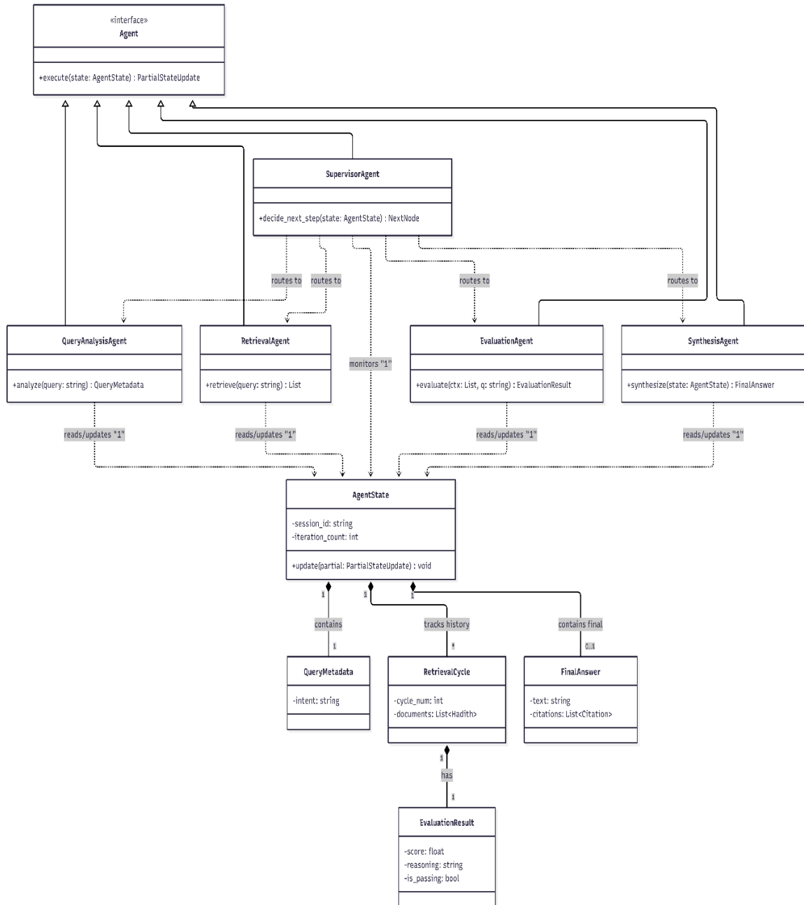
Figure 12 class diagram
