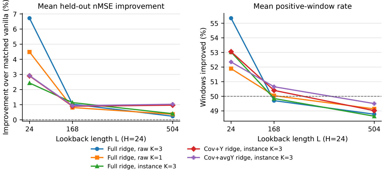
Figure 1: Baseline lookback-length ablation. Dashed references mark no nMSE improvement and a 50% window win rate.
