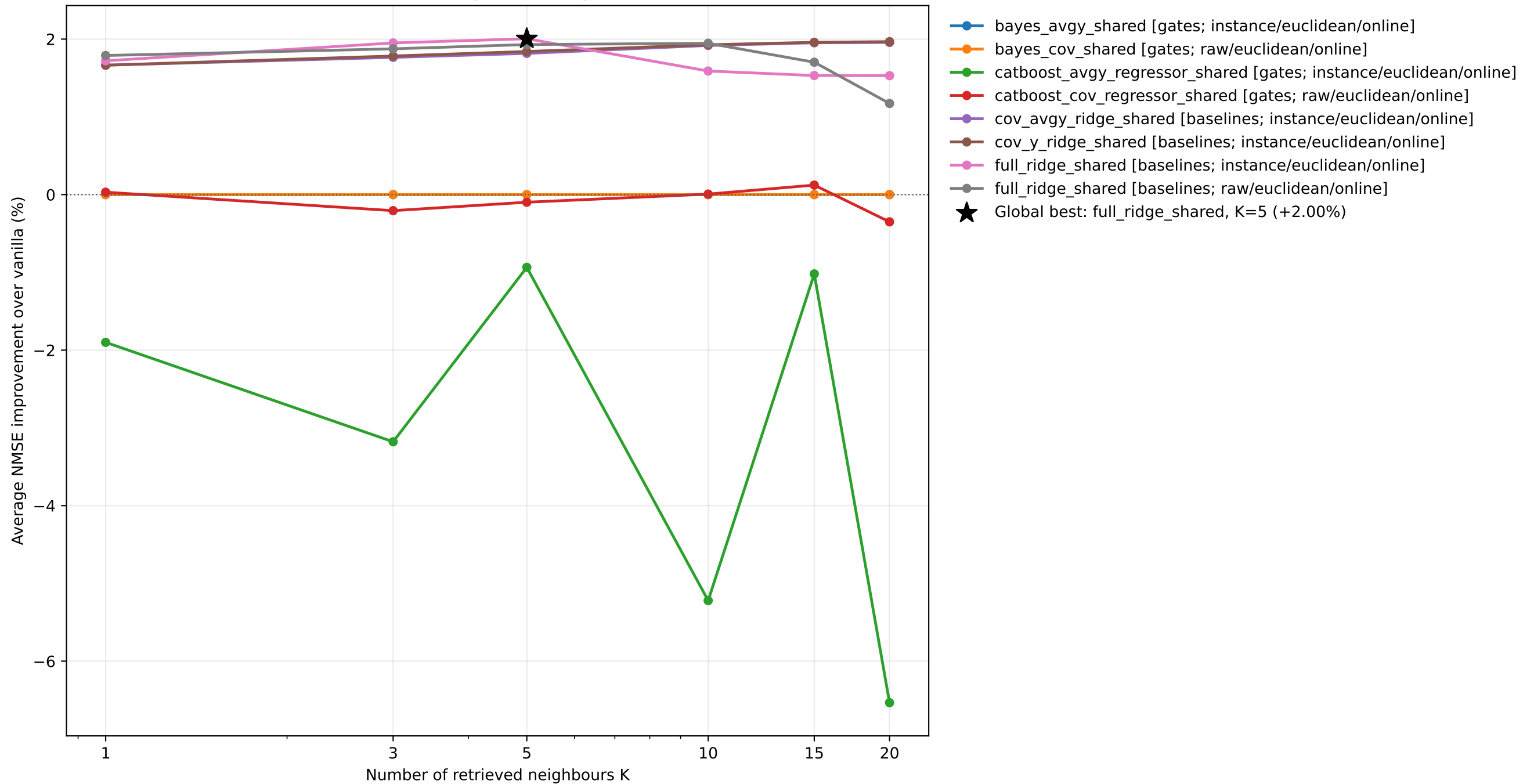
K ablation: average NMSE improvement
