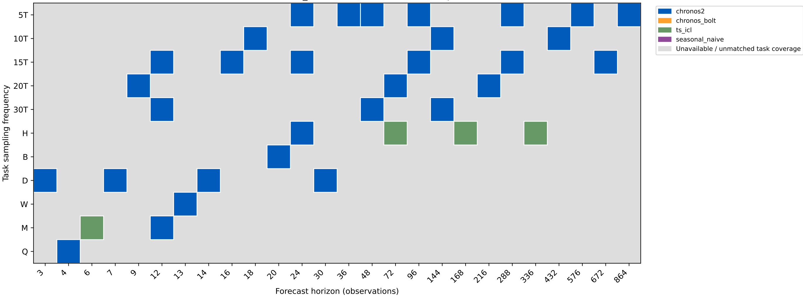
Best Mean task MASE / seasonal_naive on identical task sets; split colors = ties
