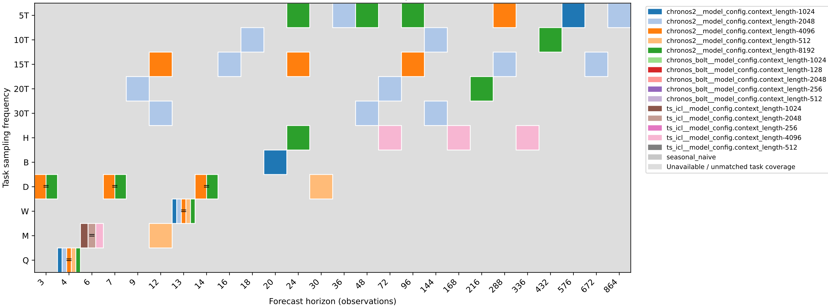
Best mean task MASE on identical task sets; split colors = ties
