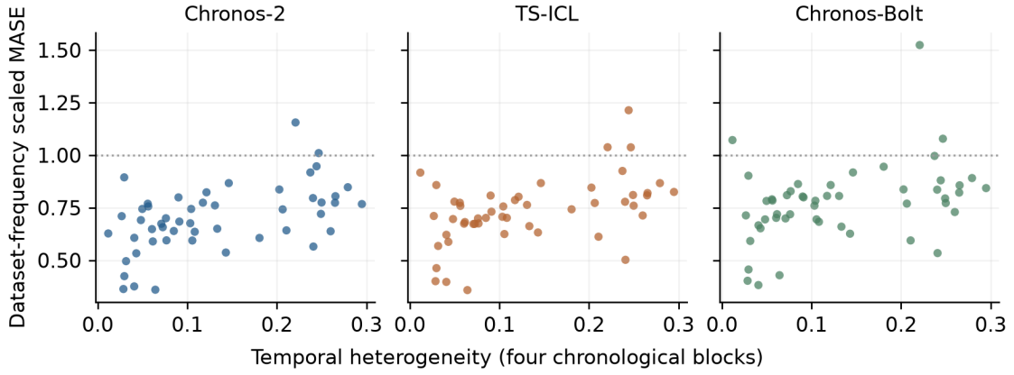
Figure 4: Temporal heterogeneity versus configuration sMASE; 50 points per model. The dotted line marks Seasonal parity.
