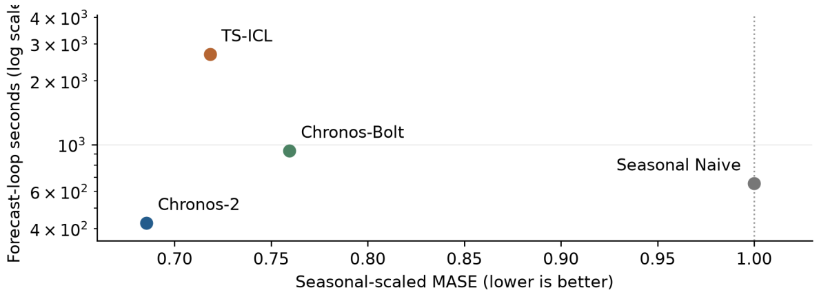
Figure 1: Accuracy and total recorded forecast-loop time on the 98 tasks. Lower and left is preferable. Time includes loop preparation but excludes model loading, metric computation, and saving.
