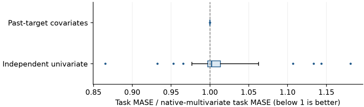
Figure 3: Task MASE divided by matched native MASE, 74 ratios per mode. Below 1 favors the alternative mode. Boxes show the middle 50% and median; whiskers span the 5th–95th percentiles, with remaining tasks shown as dots. These distributions describe differences across tasks.
