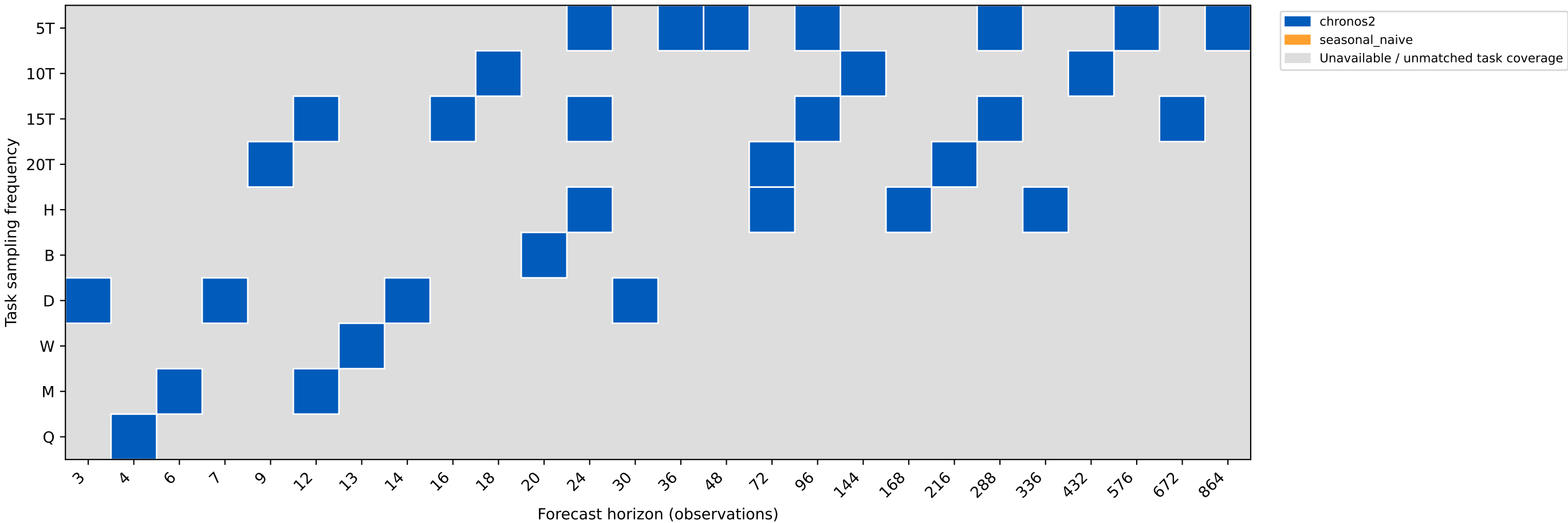
Best Mean task scaled MASE on identical task sets; split colors = ties
