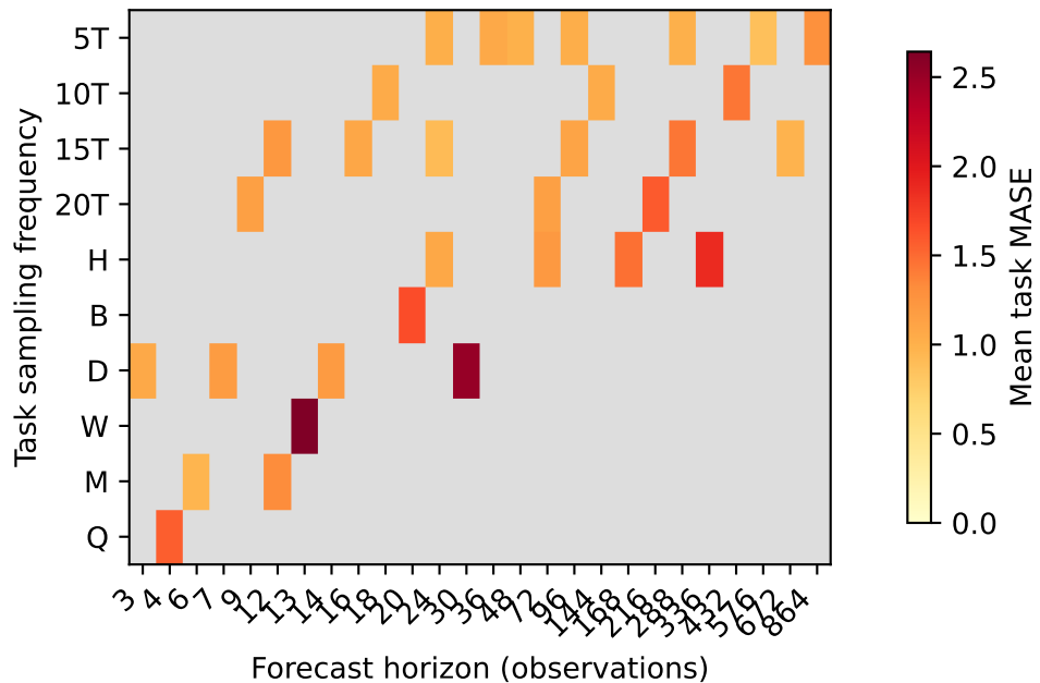
seasonal_naive
