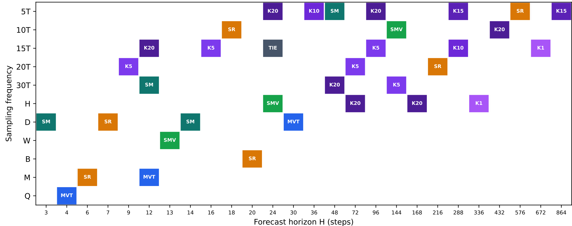
Best model by frequency and forecast horizon
