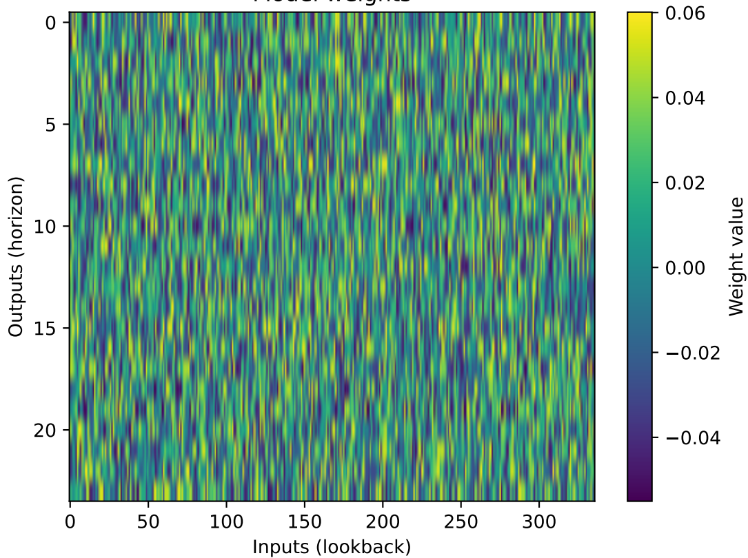
Model weights
