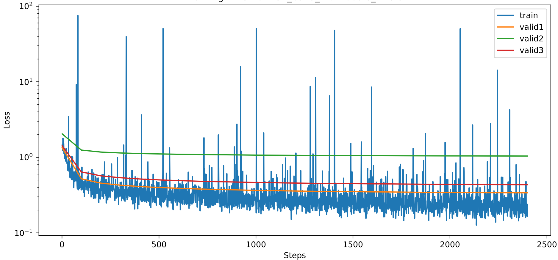
Training NMSE of TST_bs28_individuals_lr1e-5
