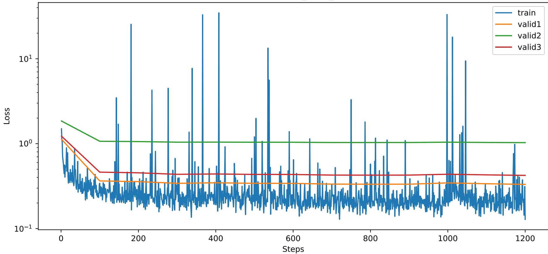
Training NMSE of TST_bs56_individuals
