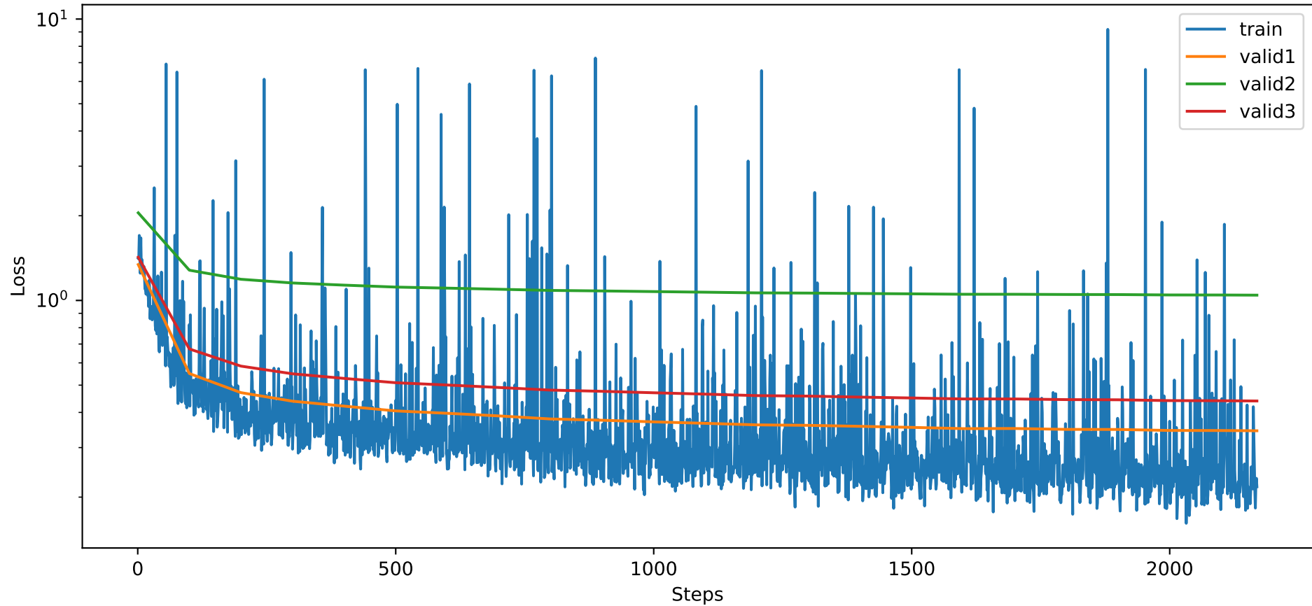
Training NMSE of TST_dates
